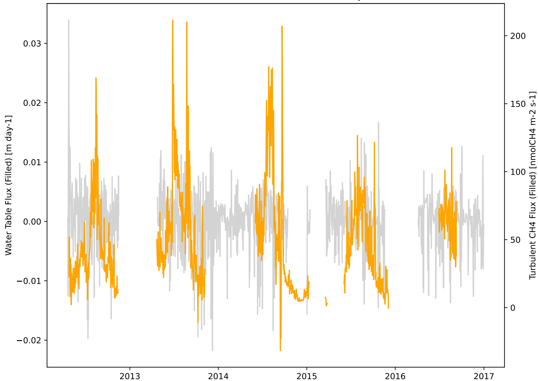
FI-Si2 Site, WTD Flux and Methane Flux Dynamics
