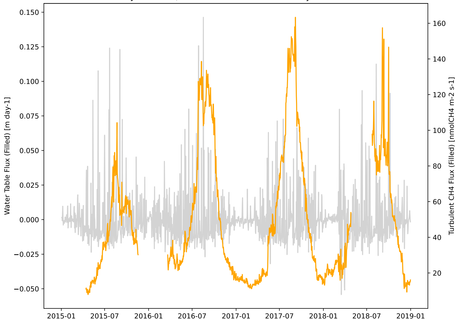
JP-BBY Site, WTD Flux and Methane Flux Dynamics
