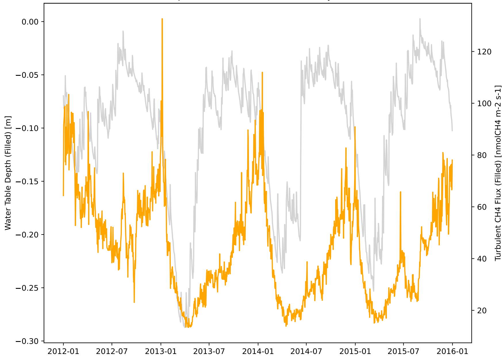
NZ-Kop Site, WTD and Methane Flux Dynamics
