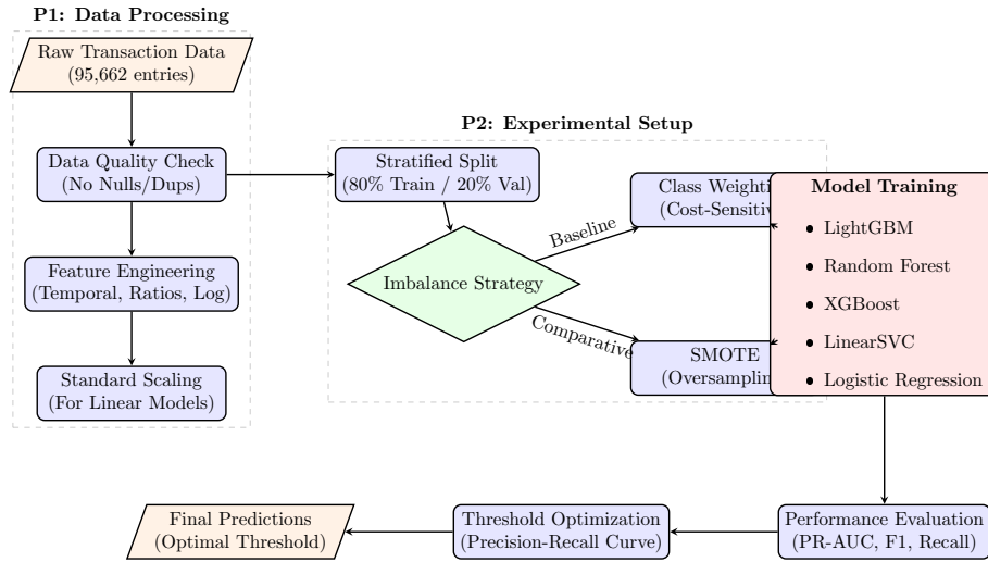
Figure 1: Methodological Workflow from Data Ingestion to Model Optimisation
