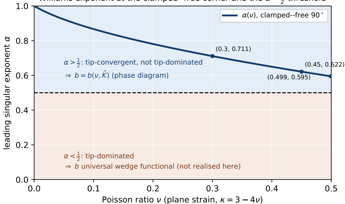
Williams exponent at the clamped--free corner and the \alpha = \frac{1}{2} threshold
