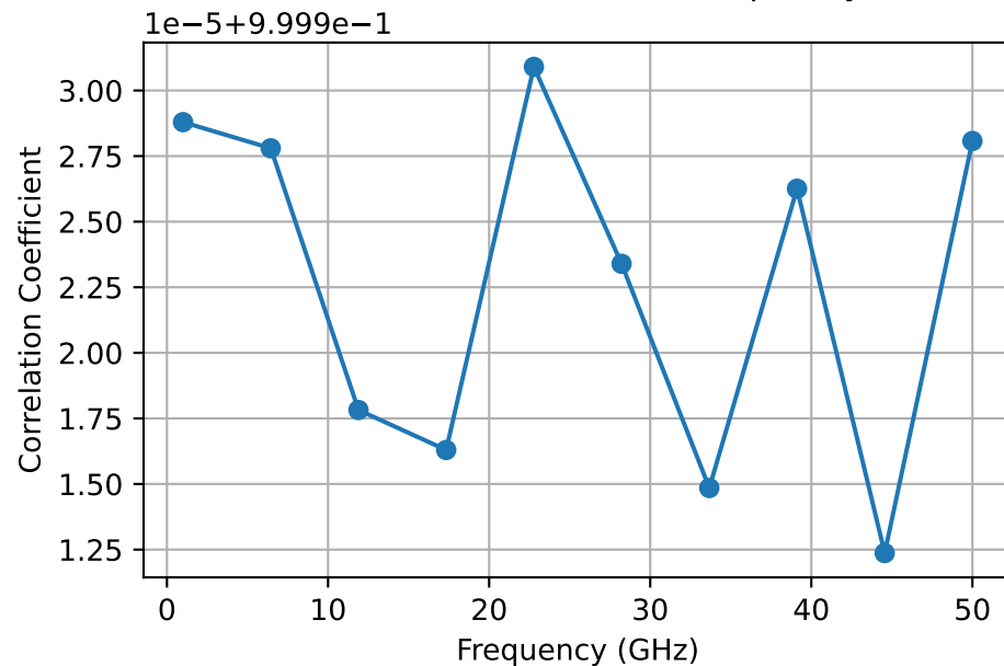
Pattern Correlation vs Frequency
