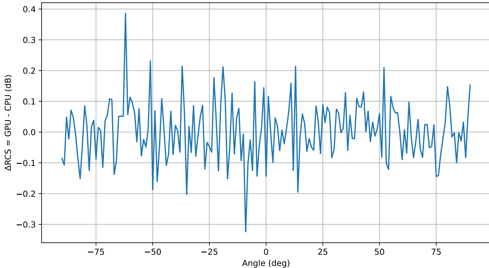
Difference Plot ( \Delta RCS vs Angle) @ 6.444 GHz
