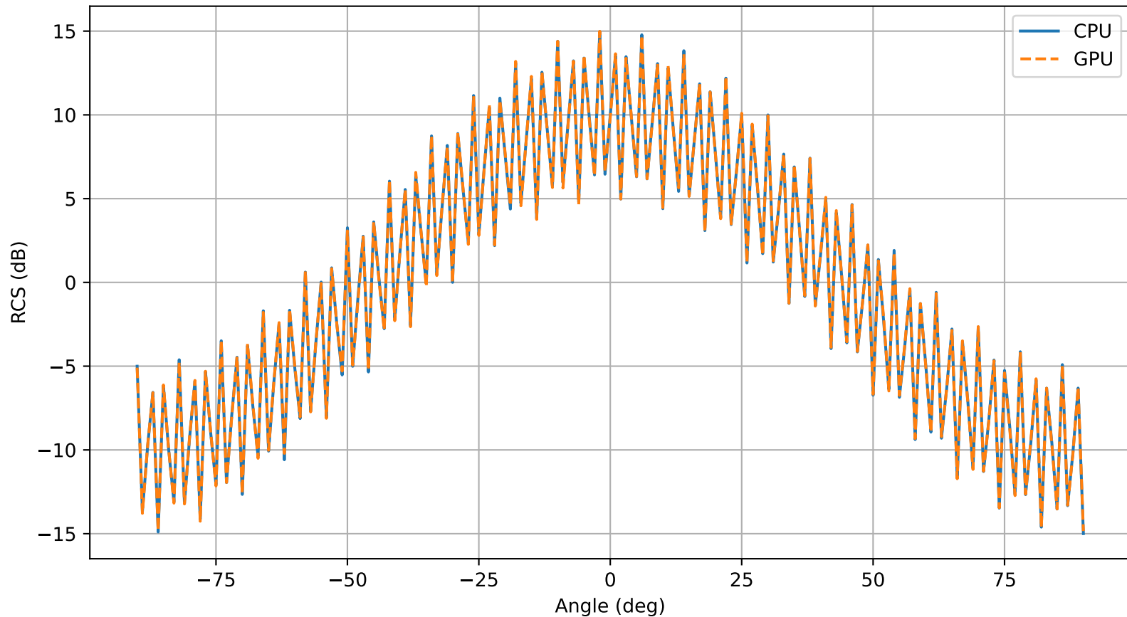
CPU vs GPU RCS Comparison @ 6.444 GHz
