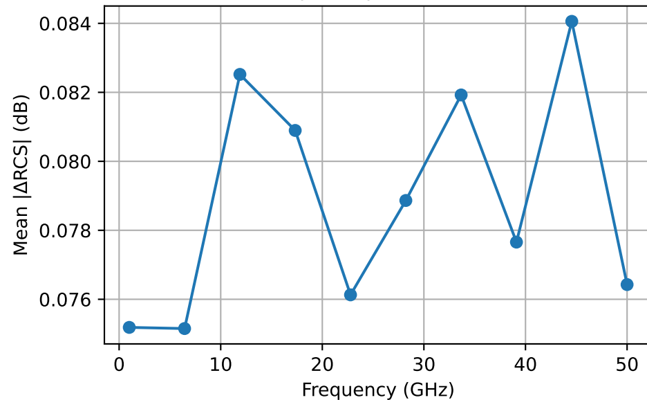
Mean |\Delta\text{RCS}| vs Frequency
