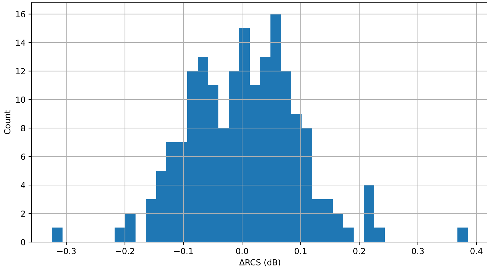
Histogram of \Delta\text{RCS} (GPU - CPU) @ 6.444 GHz
