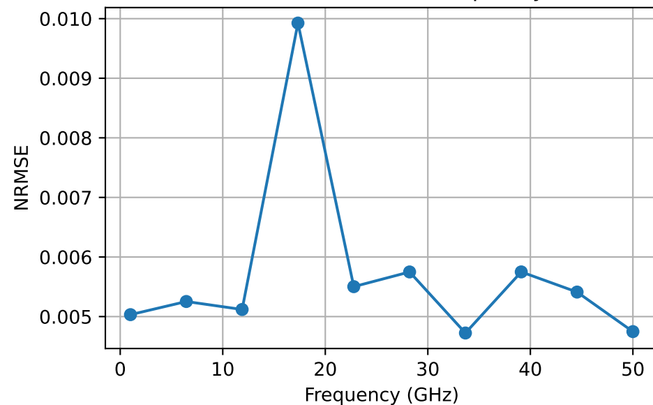
NRMSE (Linear) vs Frequency
