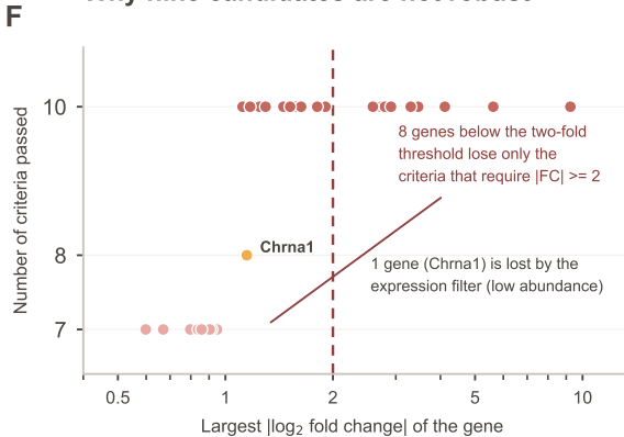
Why nine candidates are not robust
