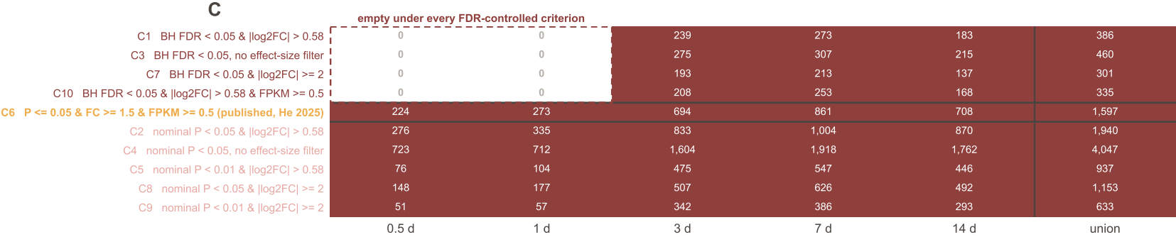
Differential-expression yield by criterion and time point
