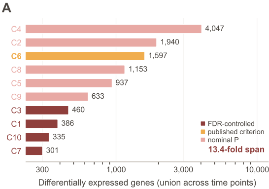
Yield of one dataset under ten analysis criteria
