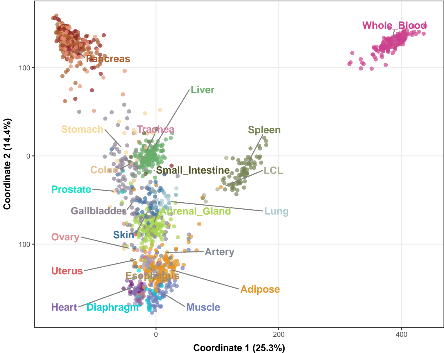
Multidimensional Scaling Analysis
