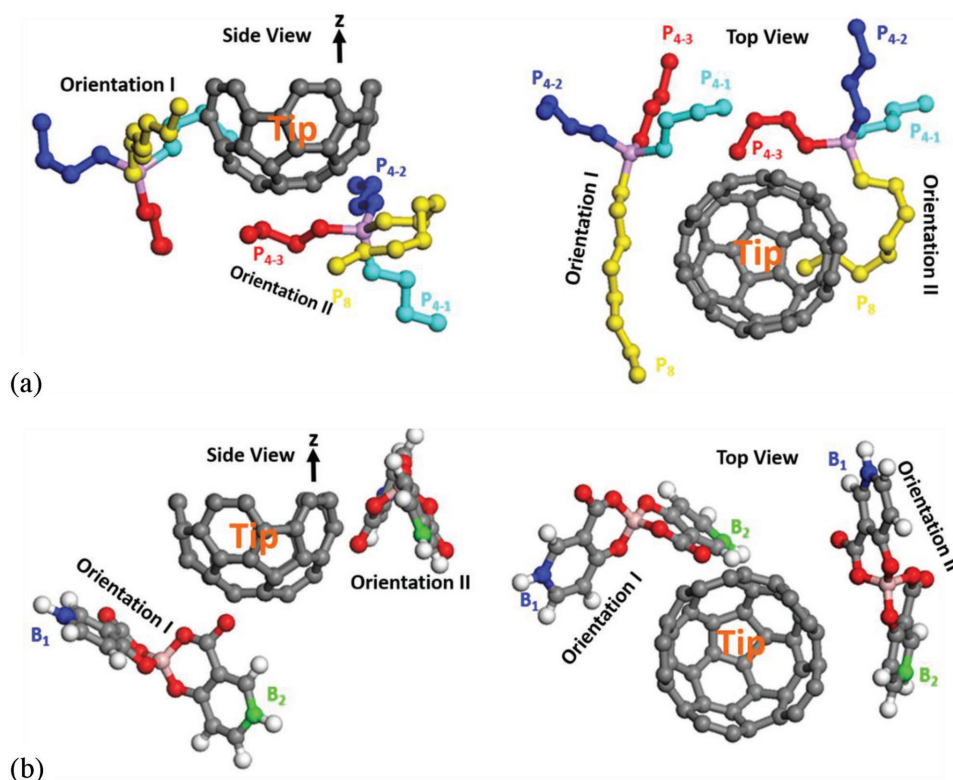
Figure 8. a,b) The sketch map showing the main orientations of P 4-1 , P 4-2 , P 4-3 , P 8 in the cation [P_{4,4,4,8}]^+ , and B 1 , B 2 in the anion [BScB]^- , respectively. Here hydrogen atoms were not shown in (a) and (b) to make the illustration more clear.
