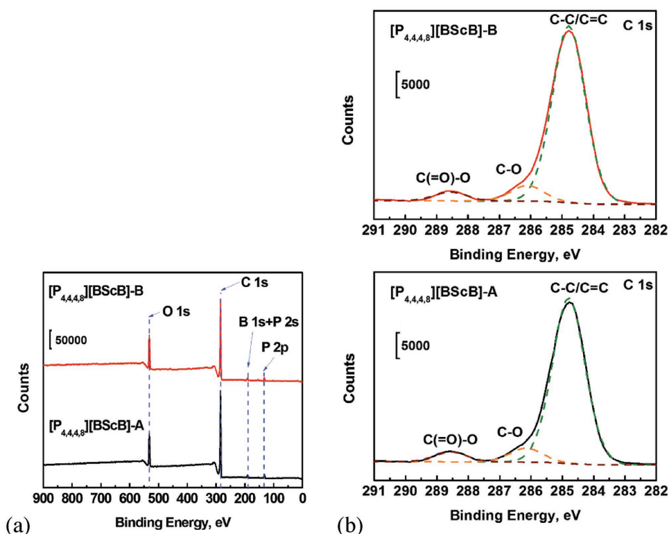
Figure 3. XPS spectra of [P_{4,4,4,8}][BScB] -oil mixtures at Ti interfaces, before ( [P_{4,4,4,8}][BScB] -B) and after ( [P_{4,4,4,8}][BScB] -A) AFM friction measurements: a) survey, b) high resolution C 1s scans.
