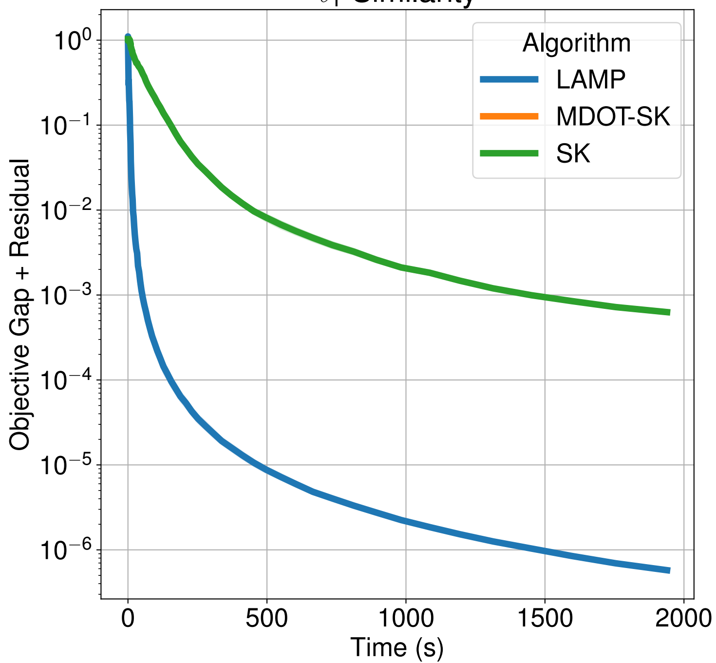
Correlation Similarity
