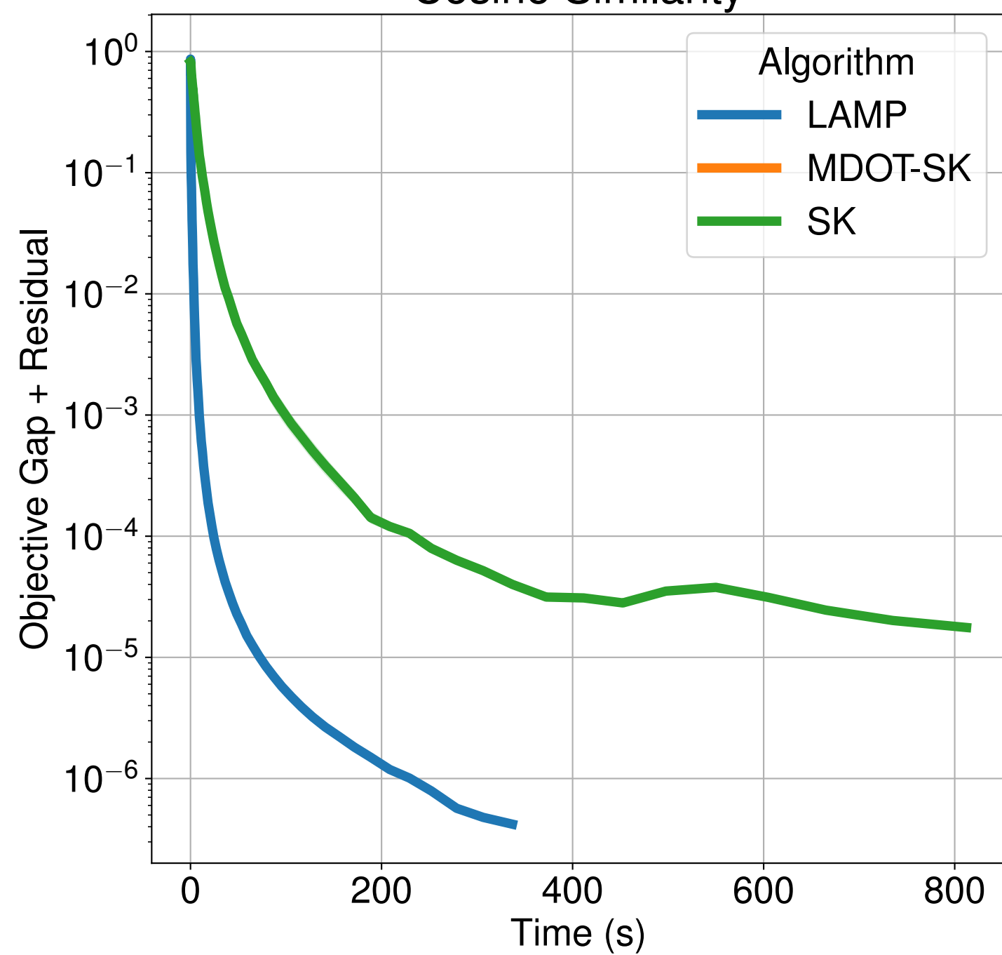
Cosine Similarity
