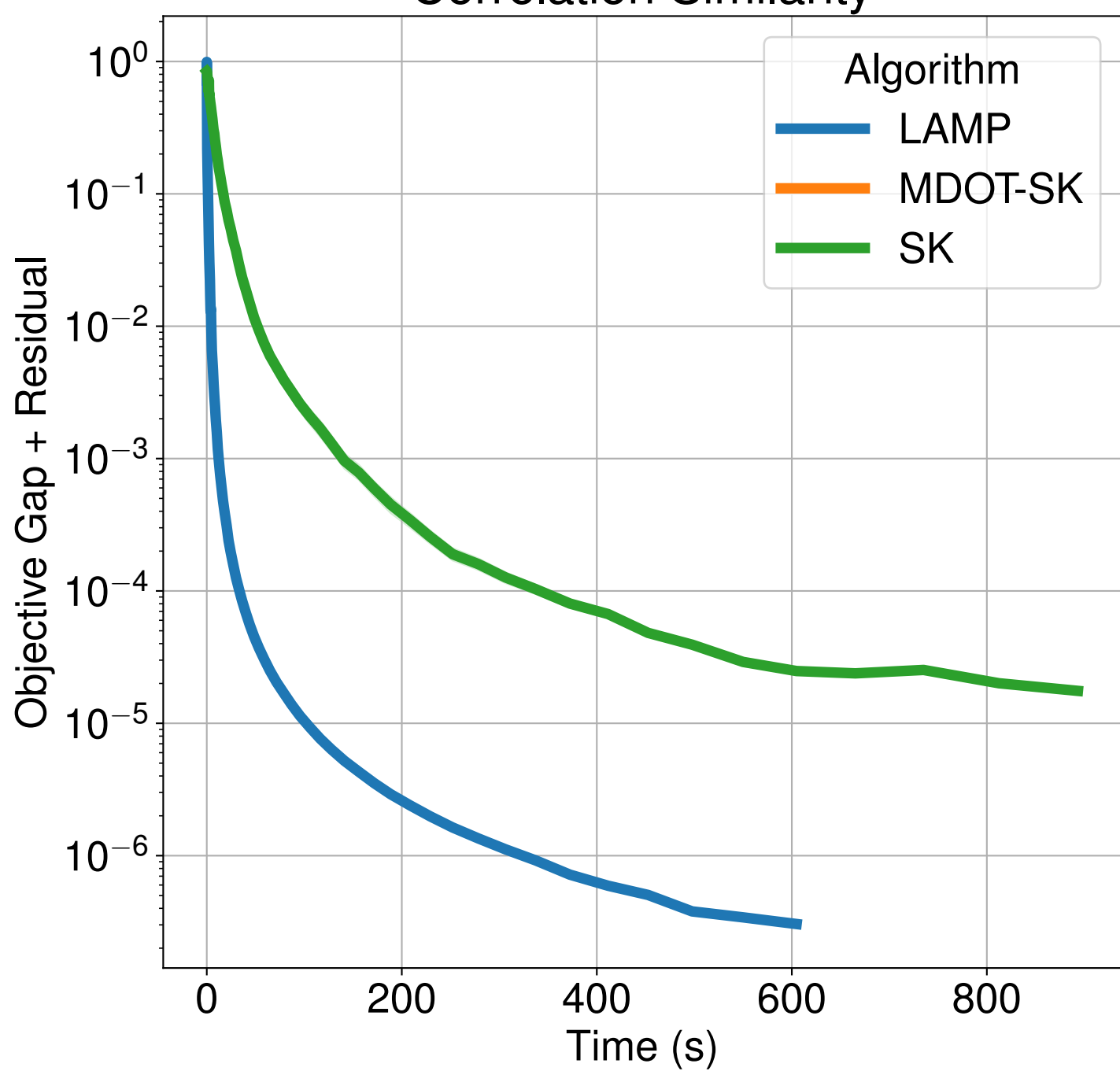
Correlation Similarity
