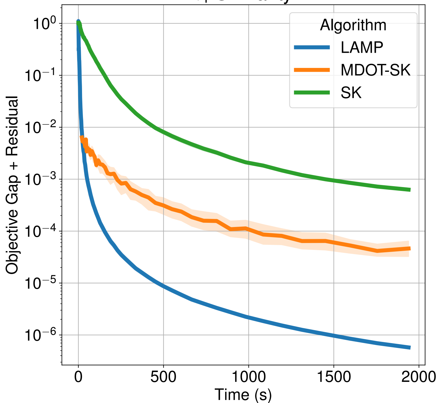
Correlation Similarity
