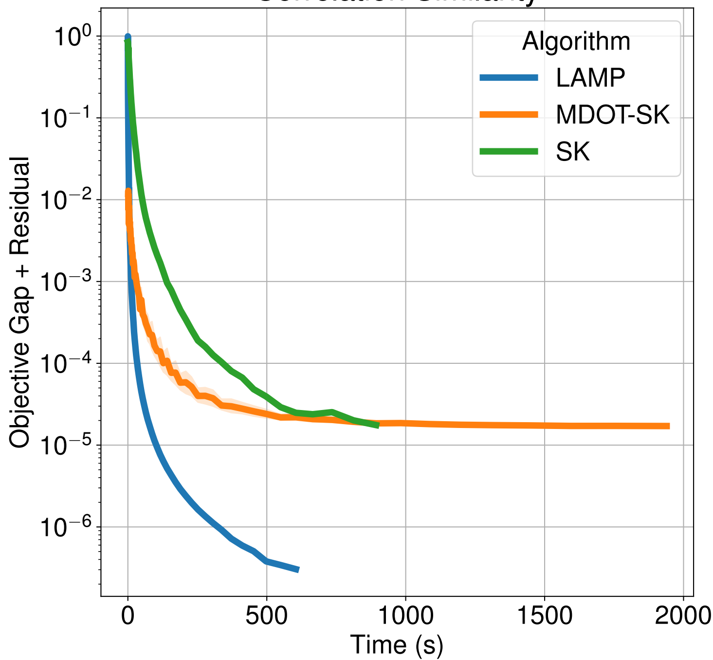
Correlation Similarity
