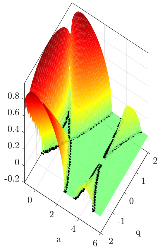
Stability Tongues \delta = 0.00
