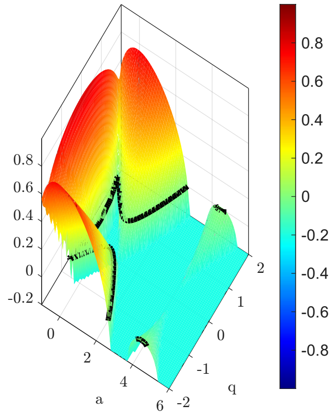
Stability Tongues \delta = 0.40
