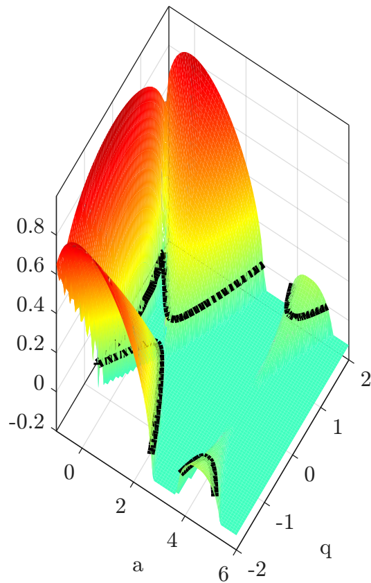
Stability Tongues \delta = 0.25
