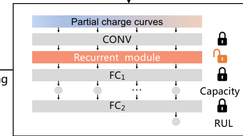
c Deep transfer learning model
