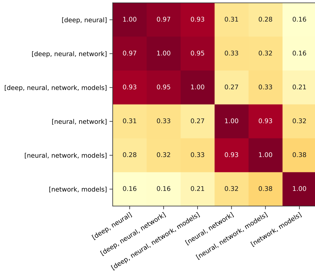
Output embedding (prefix-aligned)
