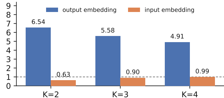
Ratio r_K = \cos_{last}/\cos_{first}
