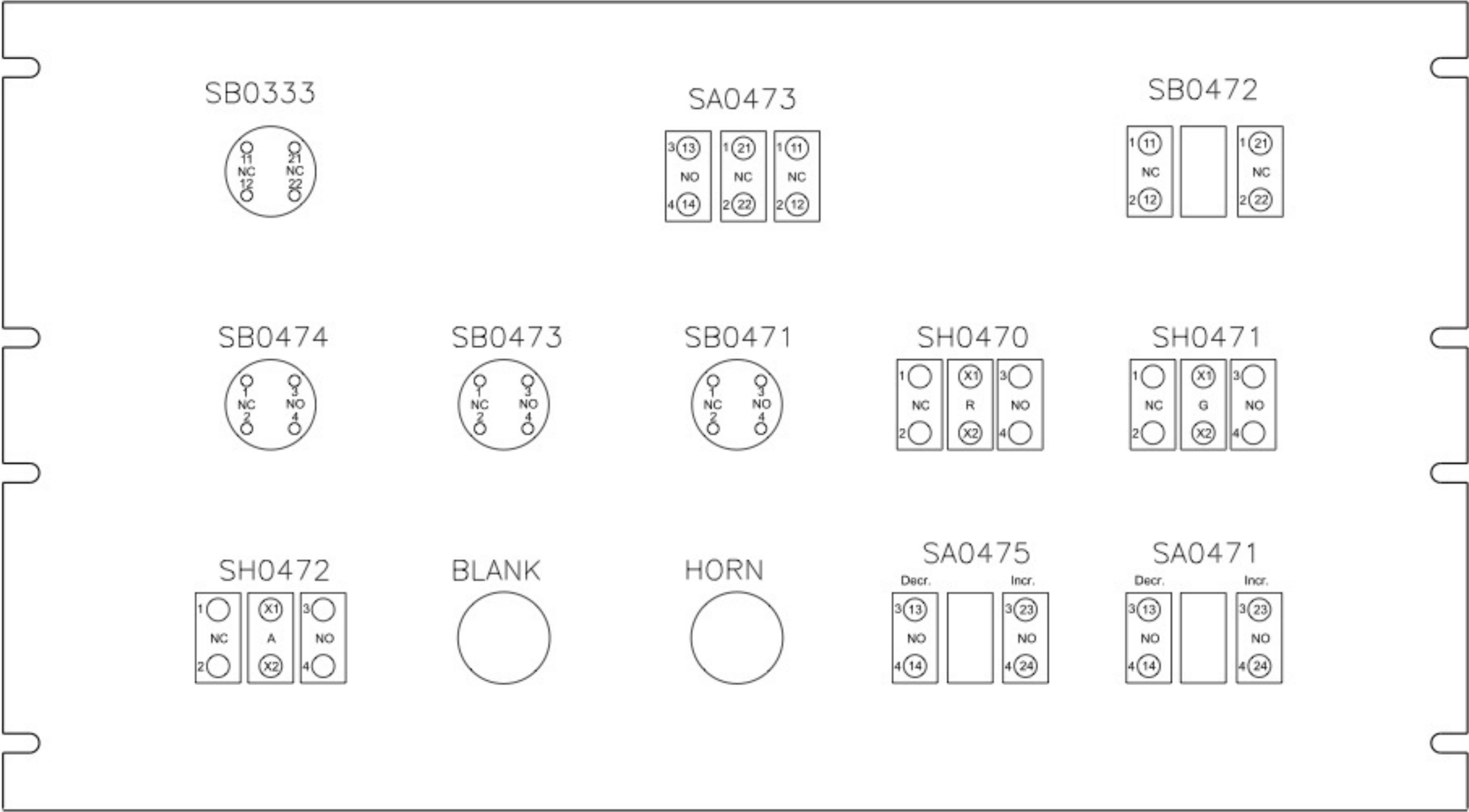
REAR VIEW
