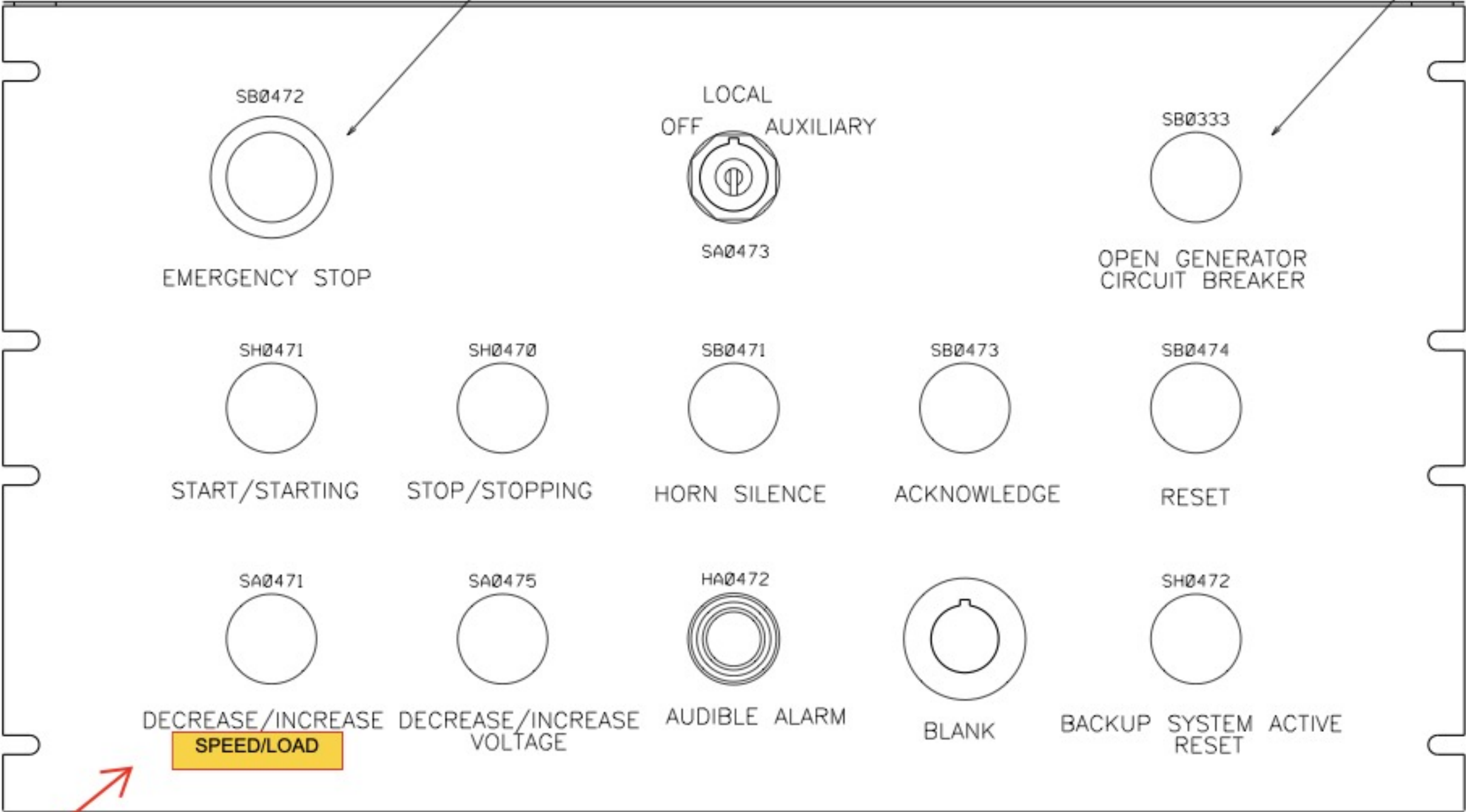
PANEL 1006616-60 OPERATOR CONTROL
