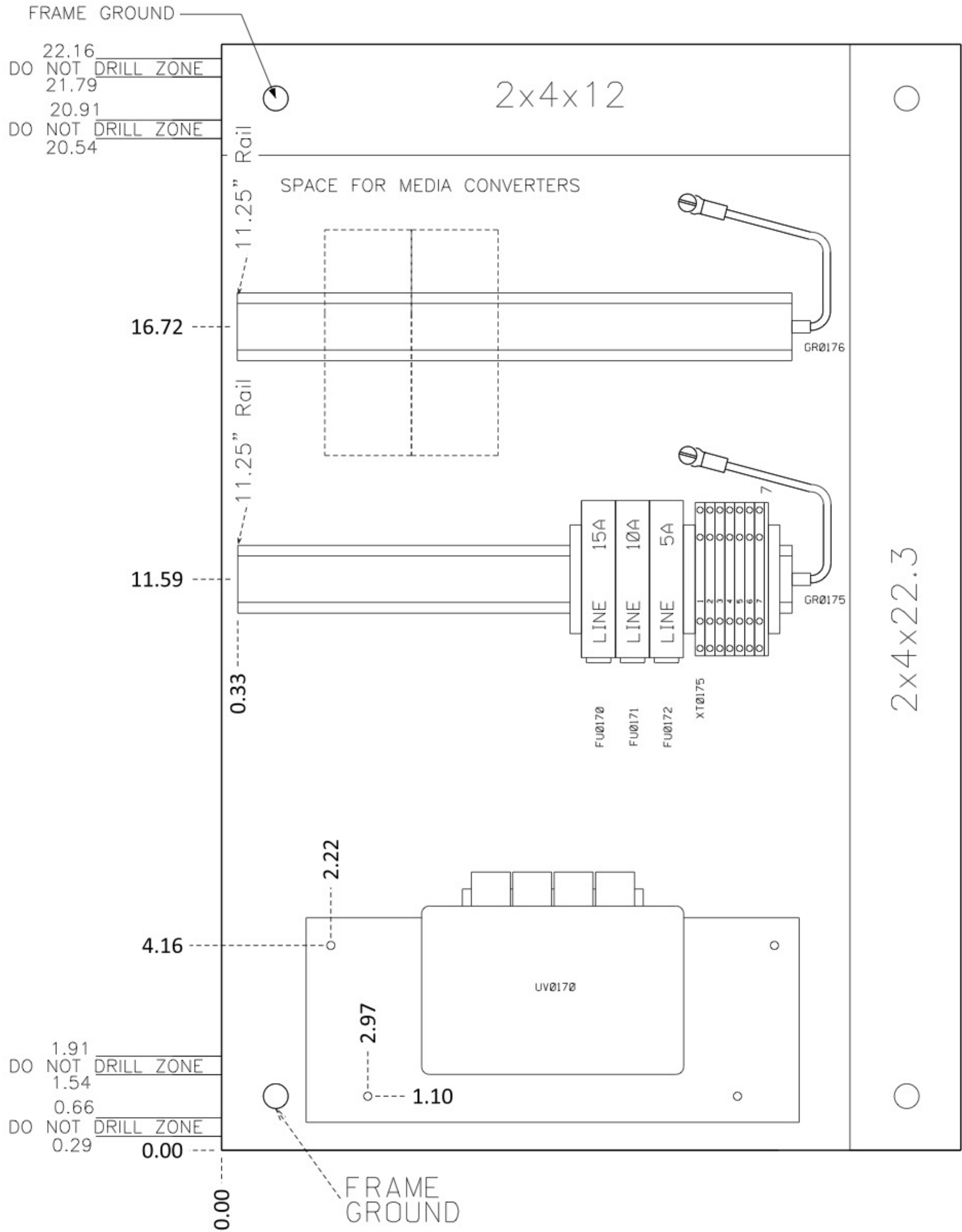
PANEL : 1702271-191 FIRE SYSTEM EQP POWER PANEL
