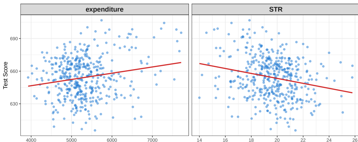
Figure 10.1 Scatter plots of TestScore vs expenditure and STR. STR stands for students-teach ratio, proxying class size.
