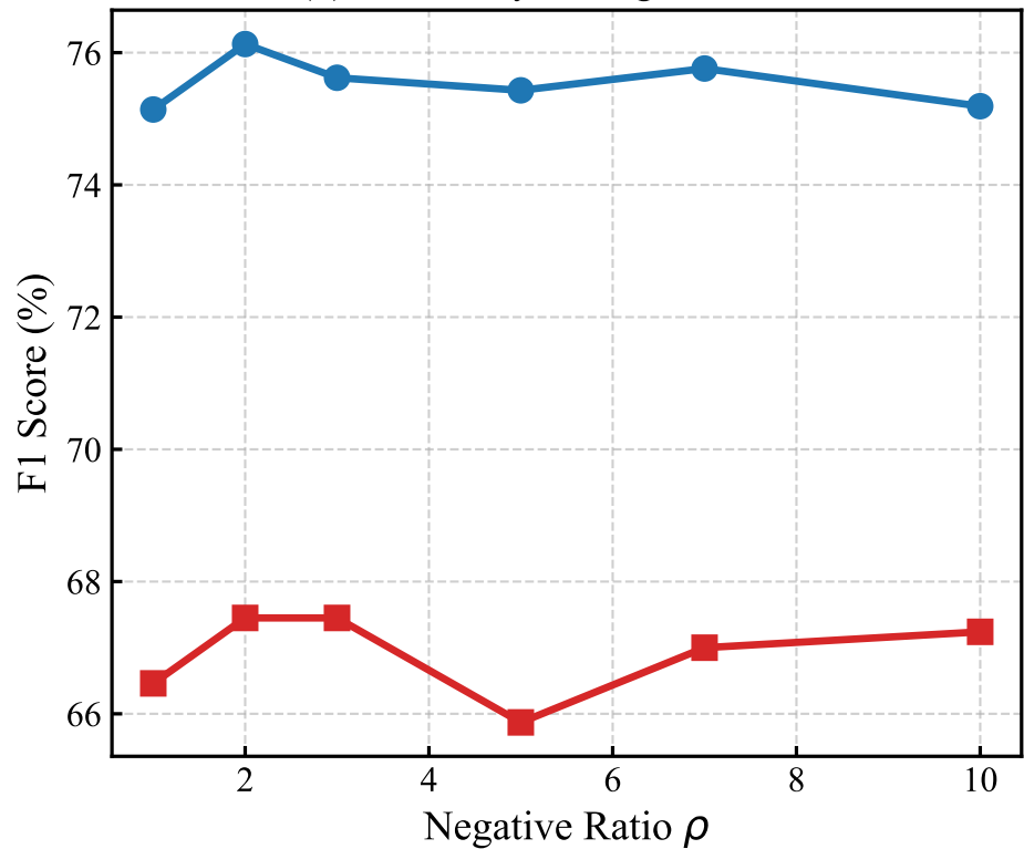
(b) Sensitivity to Negative Ratio
