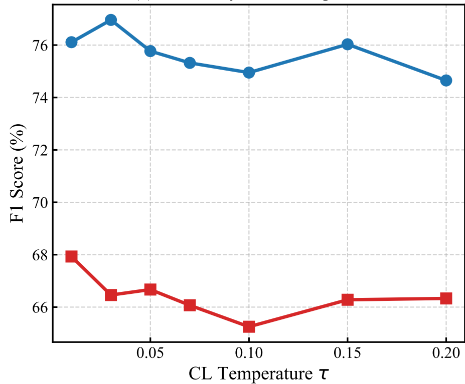
(a) Sensitivity to CL Temperature
