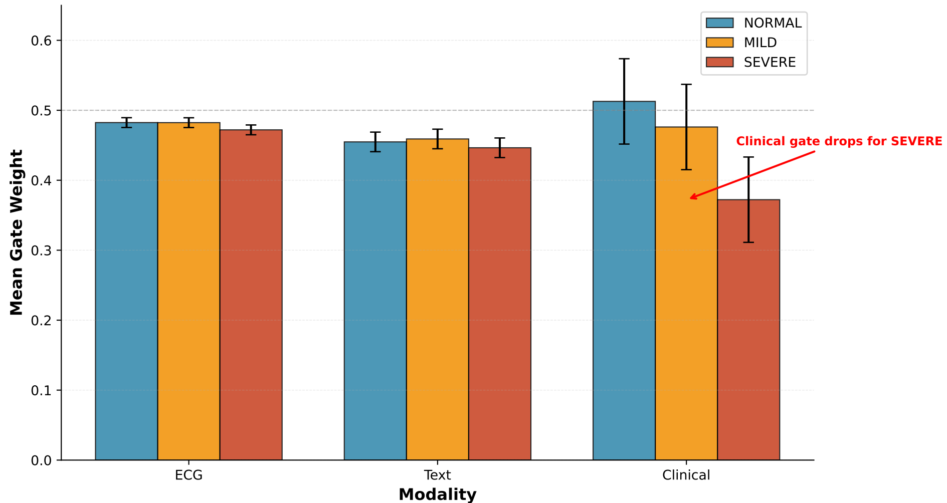
Figure 5: Context-Gated Attention (CGA) Gate Weights Range: 0 (ignore) → 1 (full pass)
