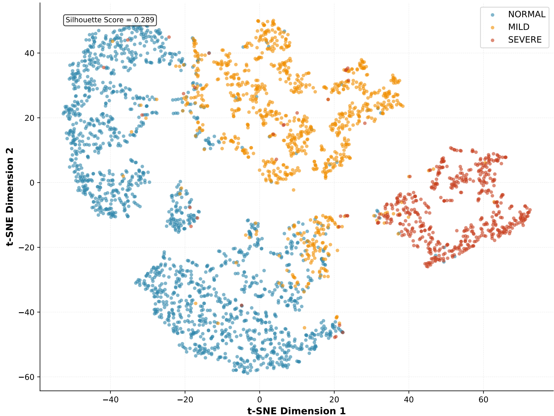
Figure 6: t-SNE Visualization of Fused Embeddings (ECG + Fine-tuned ClinicalBERT + Clinical + CGA)
