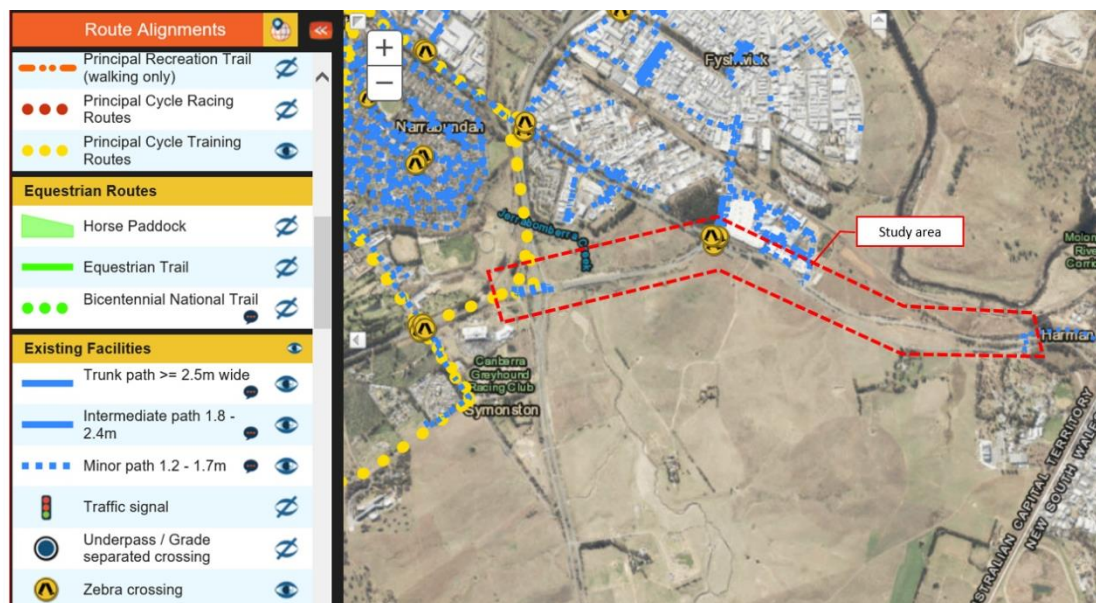
Figure 3-10 Existing walking and cycling facilities
