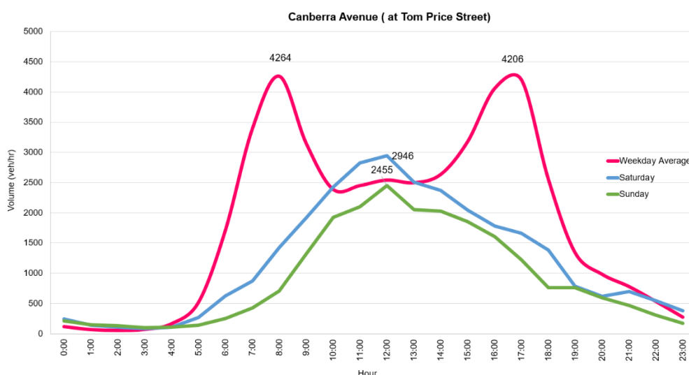
Figure 3-5 Average hourly traffic profiles – Canberra Avenue at Tom Price Street (2020)
