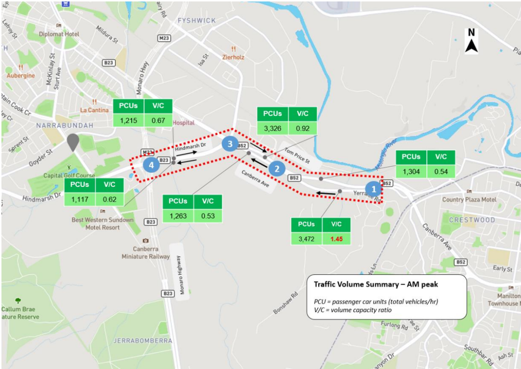
Source: Transport Canberra Map Modified by GHD Figure 5-4 Traffic volume AM peak
