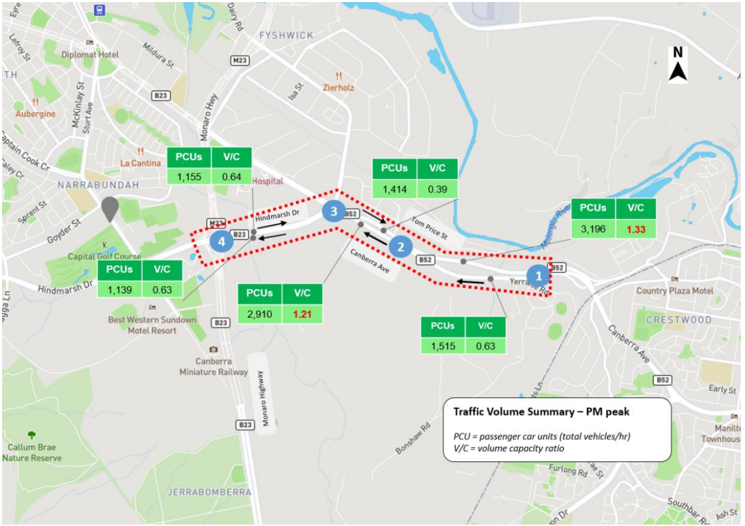
Source: Transport Canberra Map Modified by GHD Figure 5-5 Traffic volume PM peak
