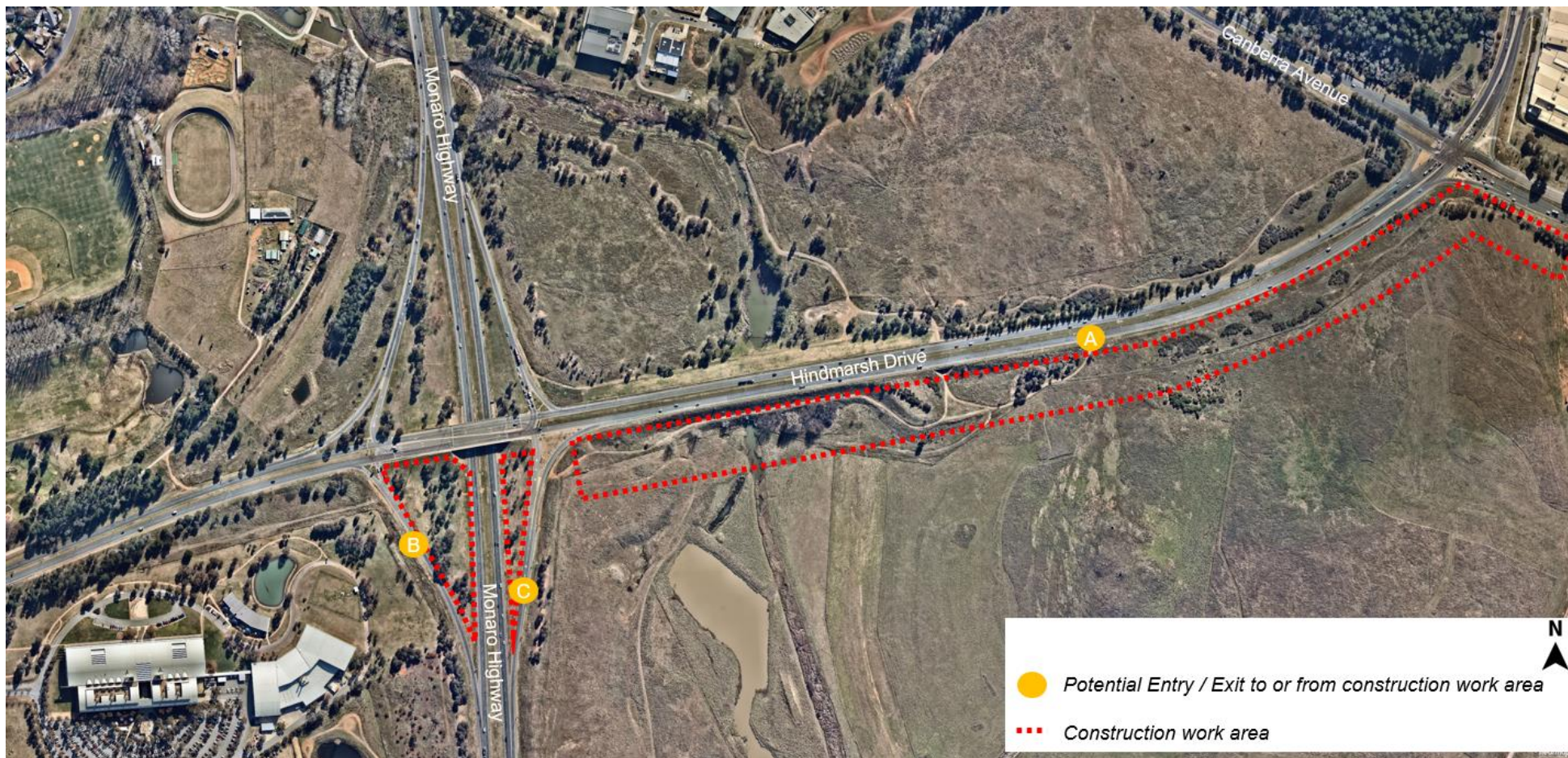
Figure 5-2 Potential Entry / Exit to or from construction work area
