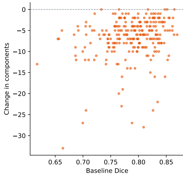
Figure E - correction benefit versus baseline quality: s2_relative_volume__frac_0.01 (exploratory)
