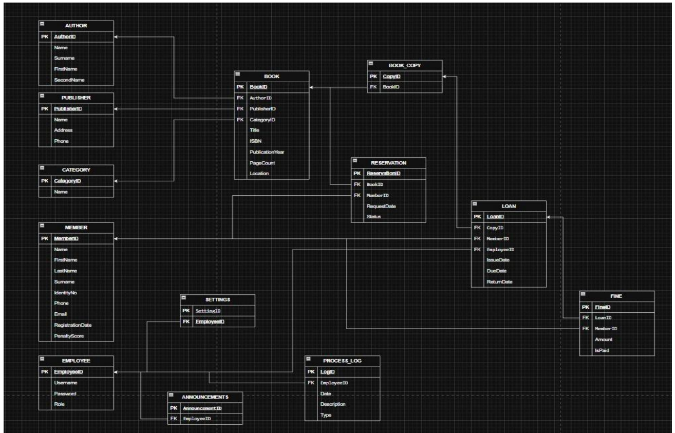
Figure 2: Detailed Relational Schema with Primary and Foreign Keys
