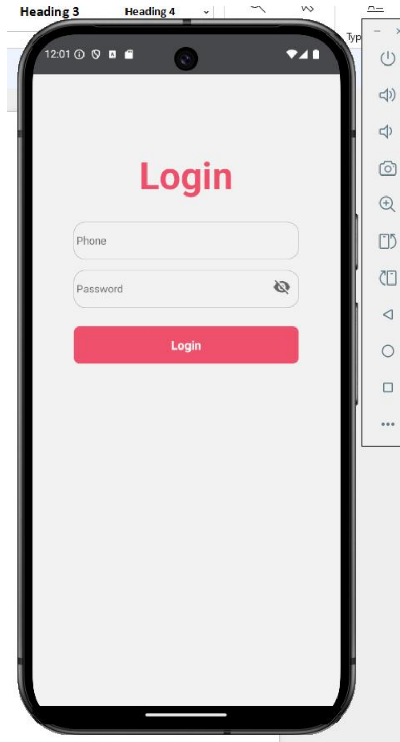
Screen 1: Login
