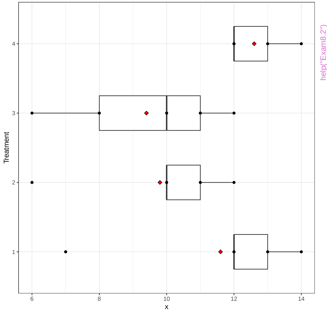
Covariate by treatment Box Plot
