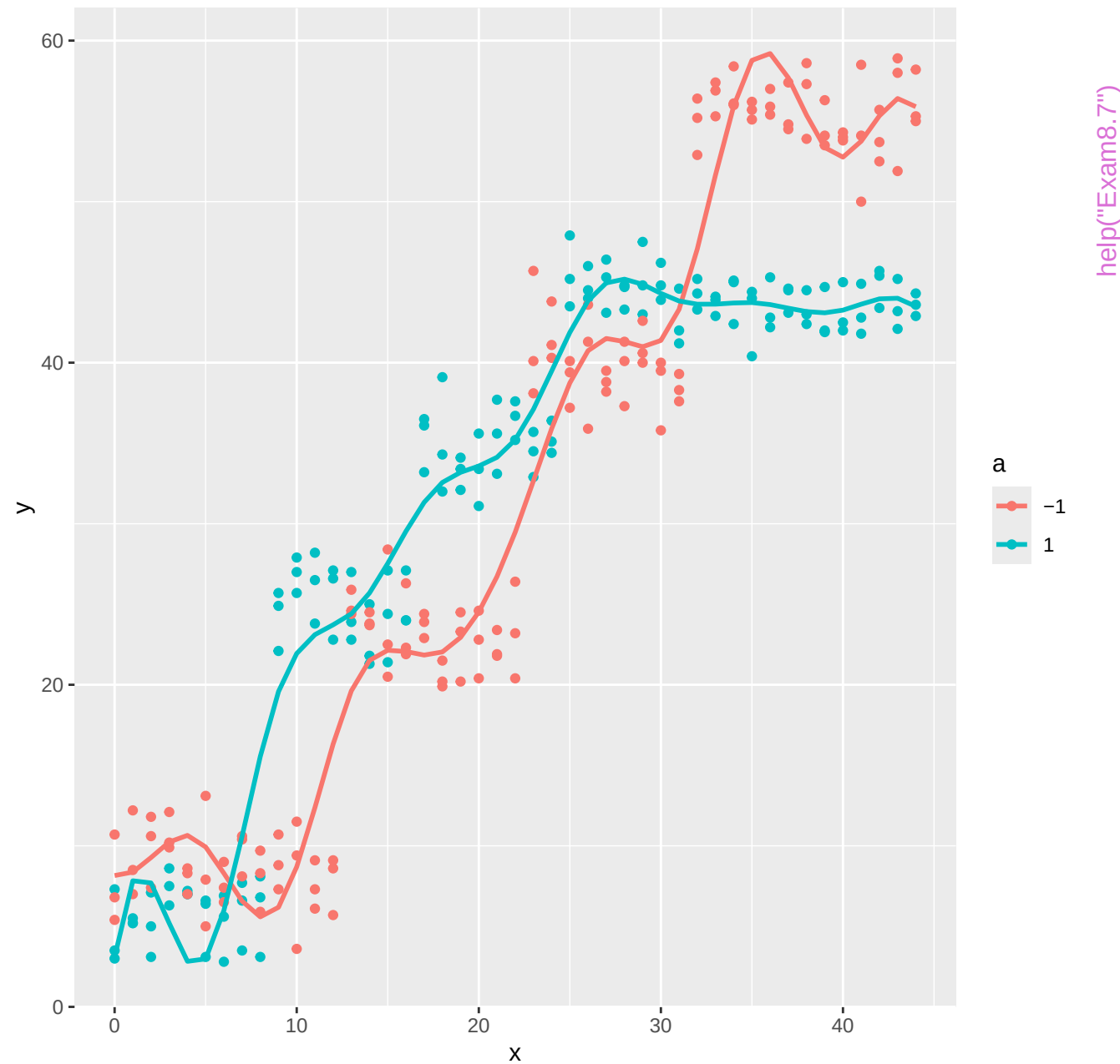
Response surface by segmented regression
