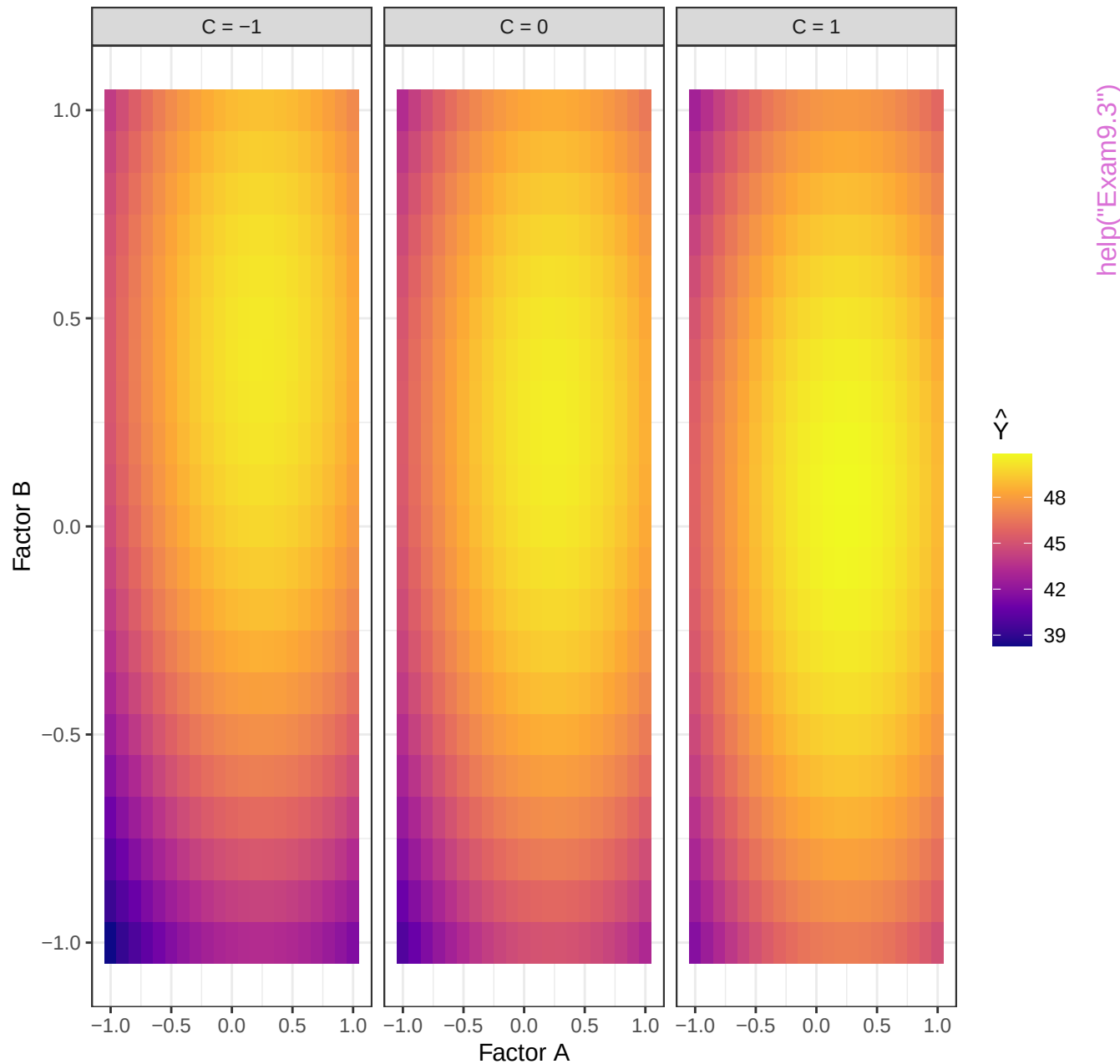
Predicted Response Surface
