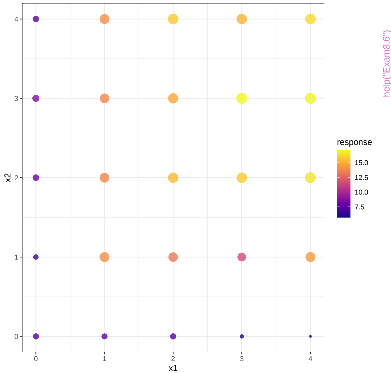
Observed Response by x1 and x2
