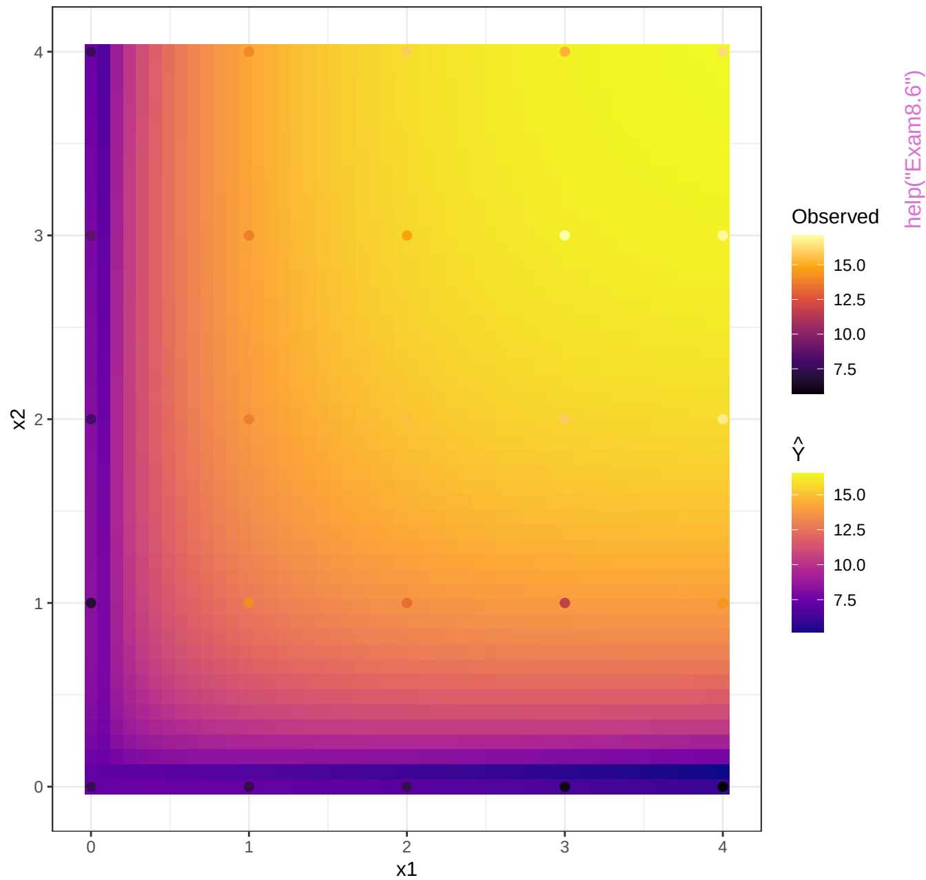
Fitted Response Surface by Hoerl Function
