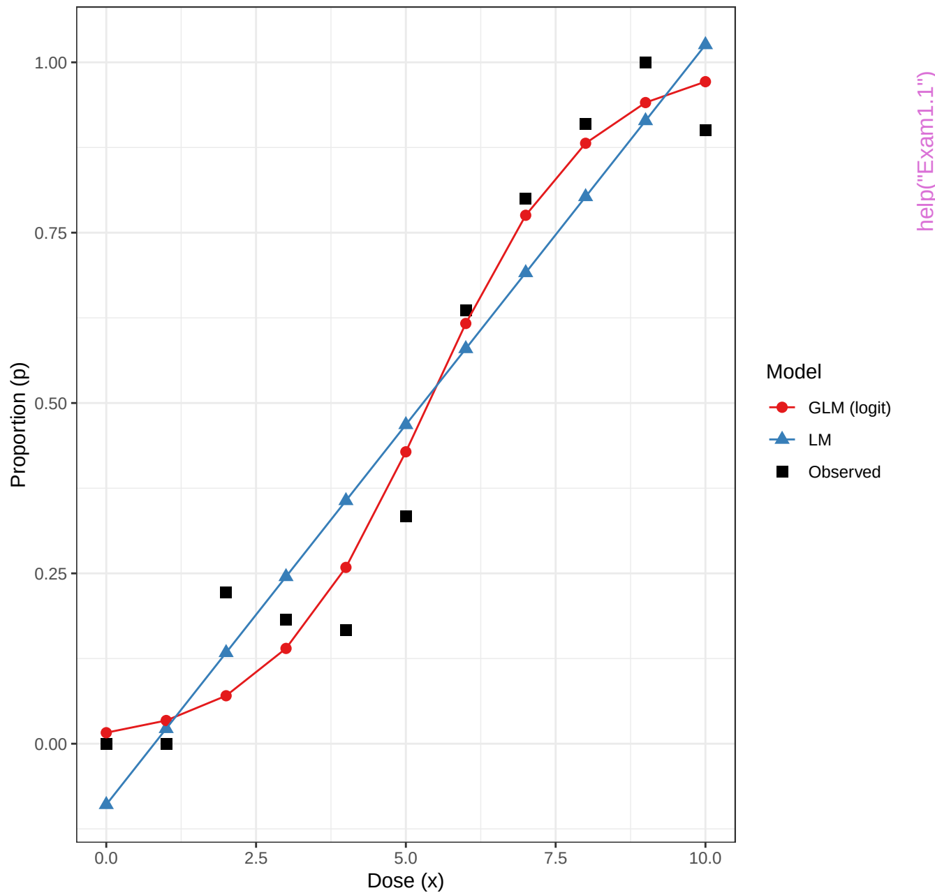
Example 1.1: Linear Model vs Logistic GLM
