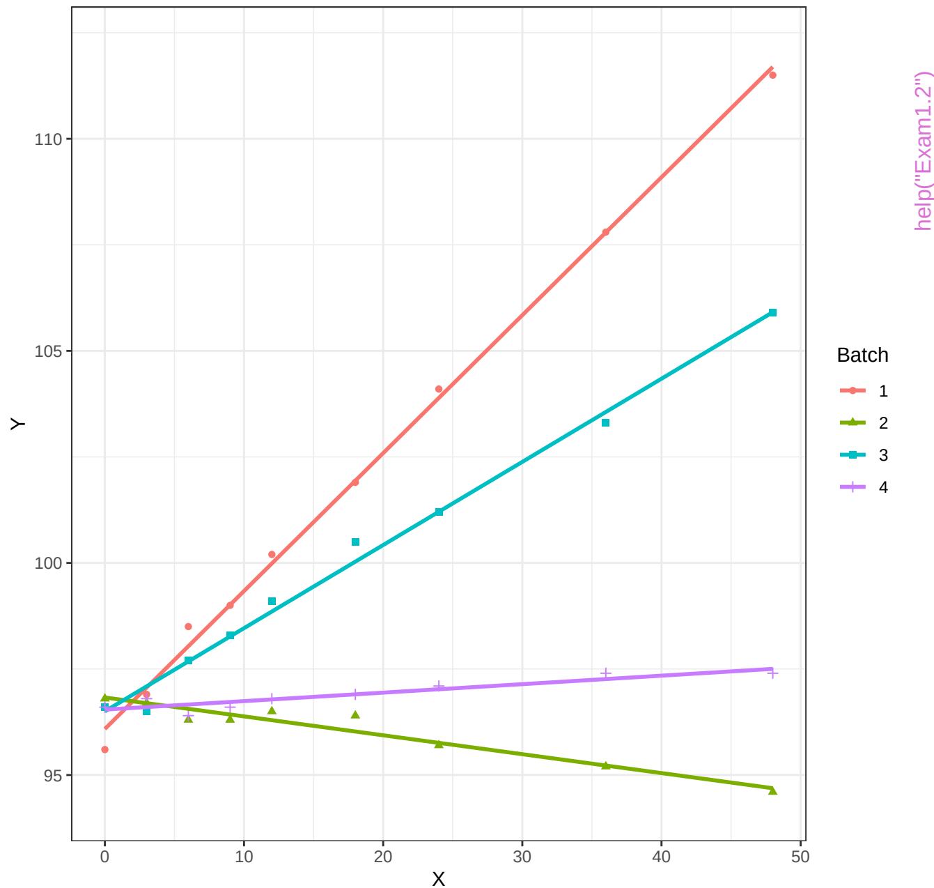
Plot of Multi Batch Regression data
