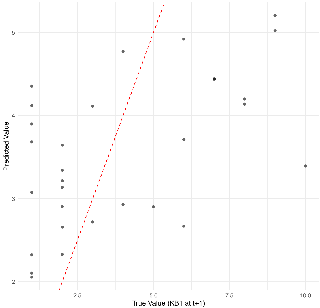
Predicted vs True for KB1
