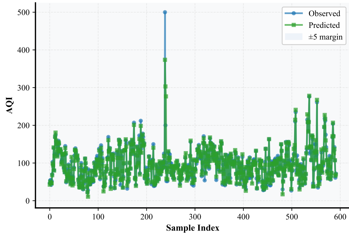
(a) Validation Set R^2 = 0.928 , RMSE = 11.501
