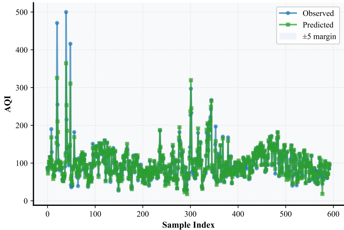
(b) Test Set R^2 = 0.934 , RMSE = 11.550
