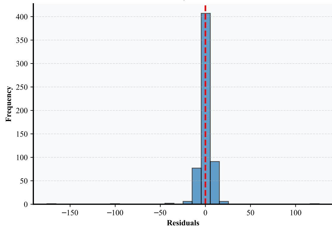
(d) Residuals Distribution (Test) Mean = 0.193, Std = 11.548
