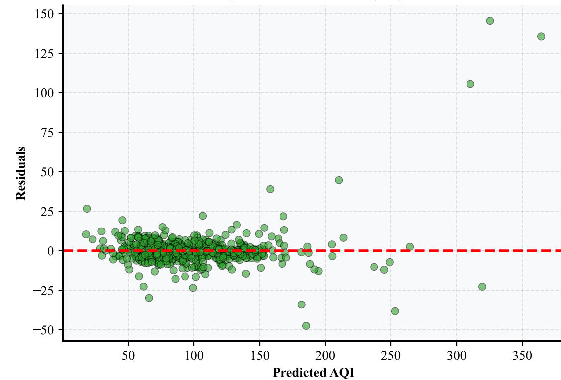
(c) Residuals vs Predicted (Test)
