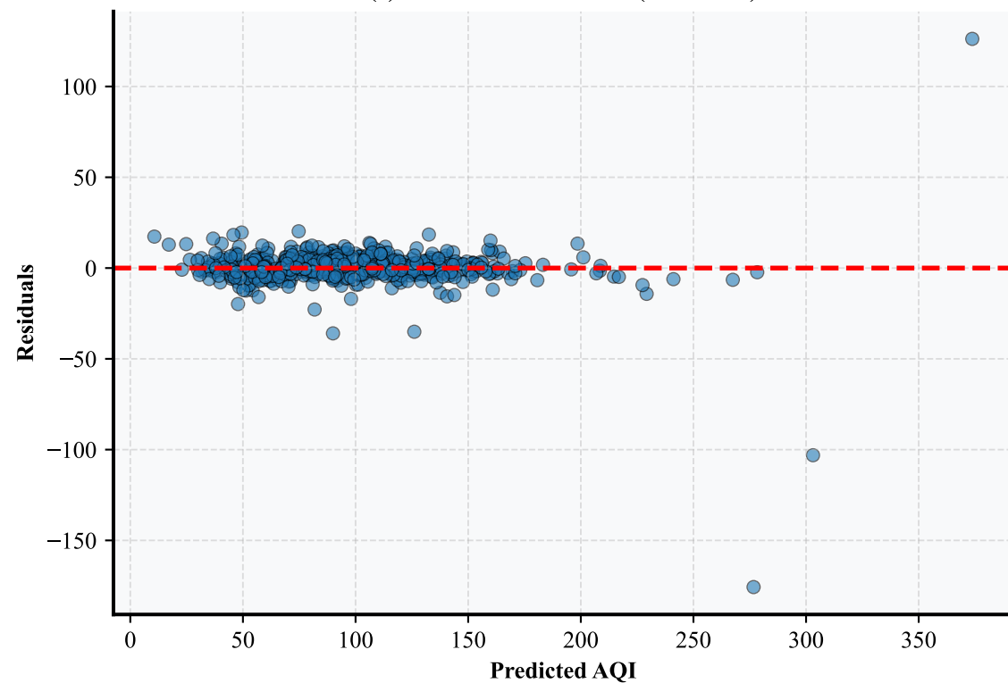
(a) Residuals vs Predicted (Validation)
