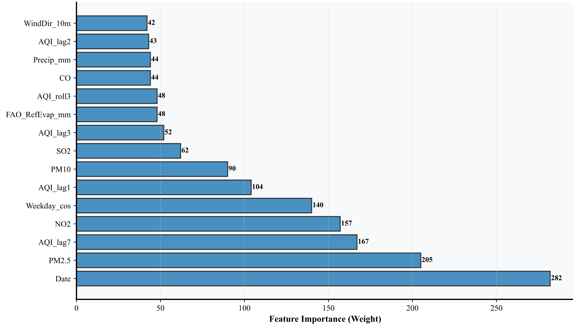
Top 15 Features by Importance
