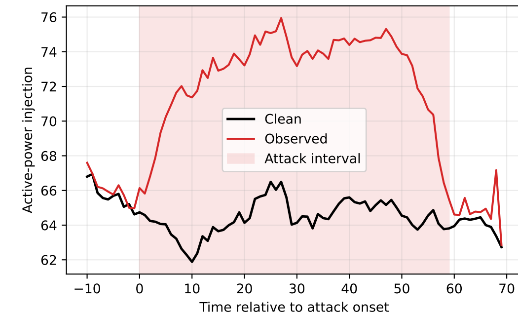
Am: observed vs. clean, bus 58
