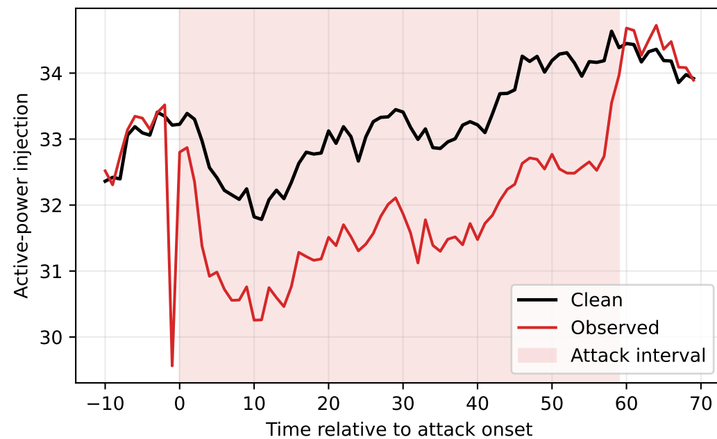
Am: observed vs. clean, bus 35
