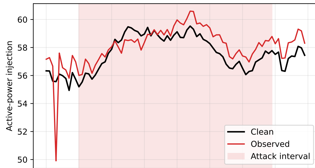
Am: observed vs. clean, bus 35
