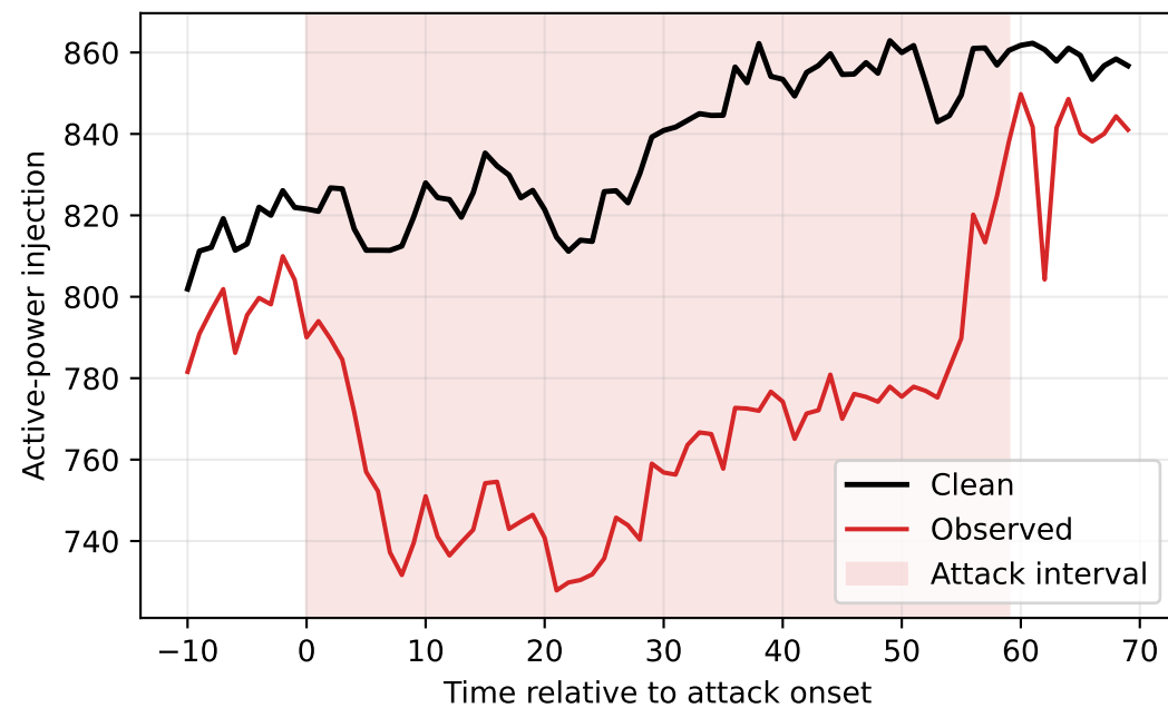
Am: observed vs. clean, bus 84
