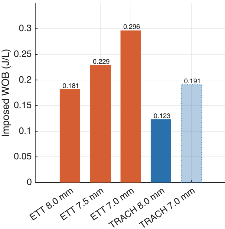
H2: imposed load at matched ventilation ( V_T = 0.45 L, RR = 18) | faded+dotted = no published coefficients
