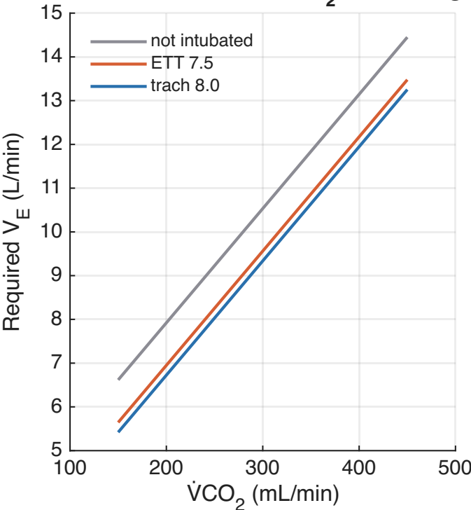
Ventilation to hold \text{PaCO}_2 = 40 \text{ mmHg}
