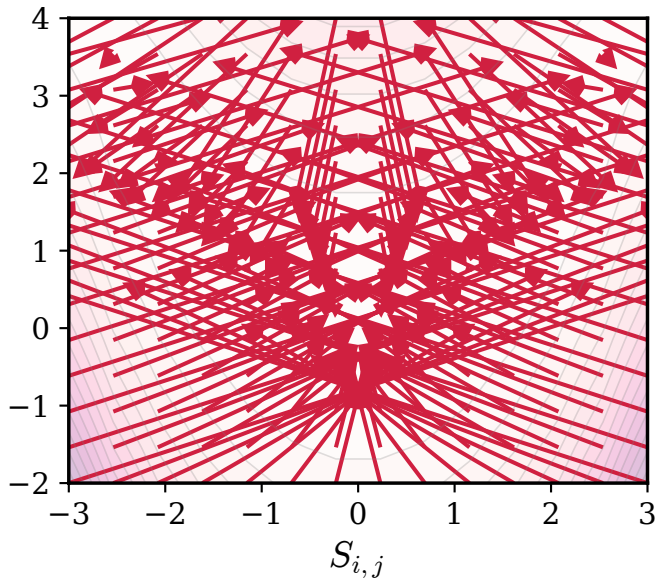
Euclidean Direction
