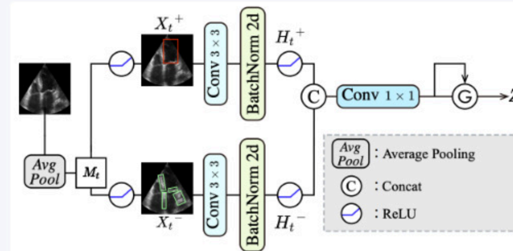
Figure 5. APFE: contrast decomposition provides noise-resilient cues.
