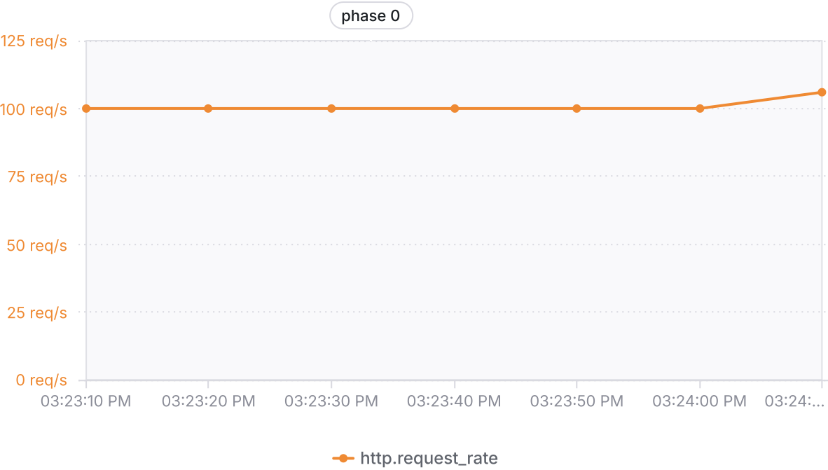
http.request_rate
