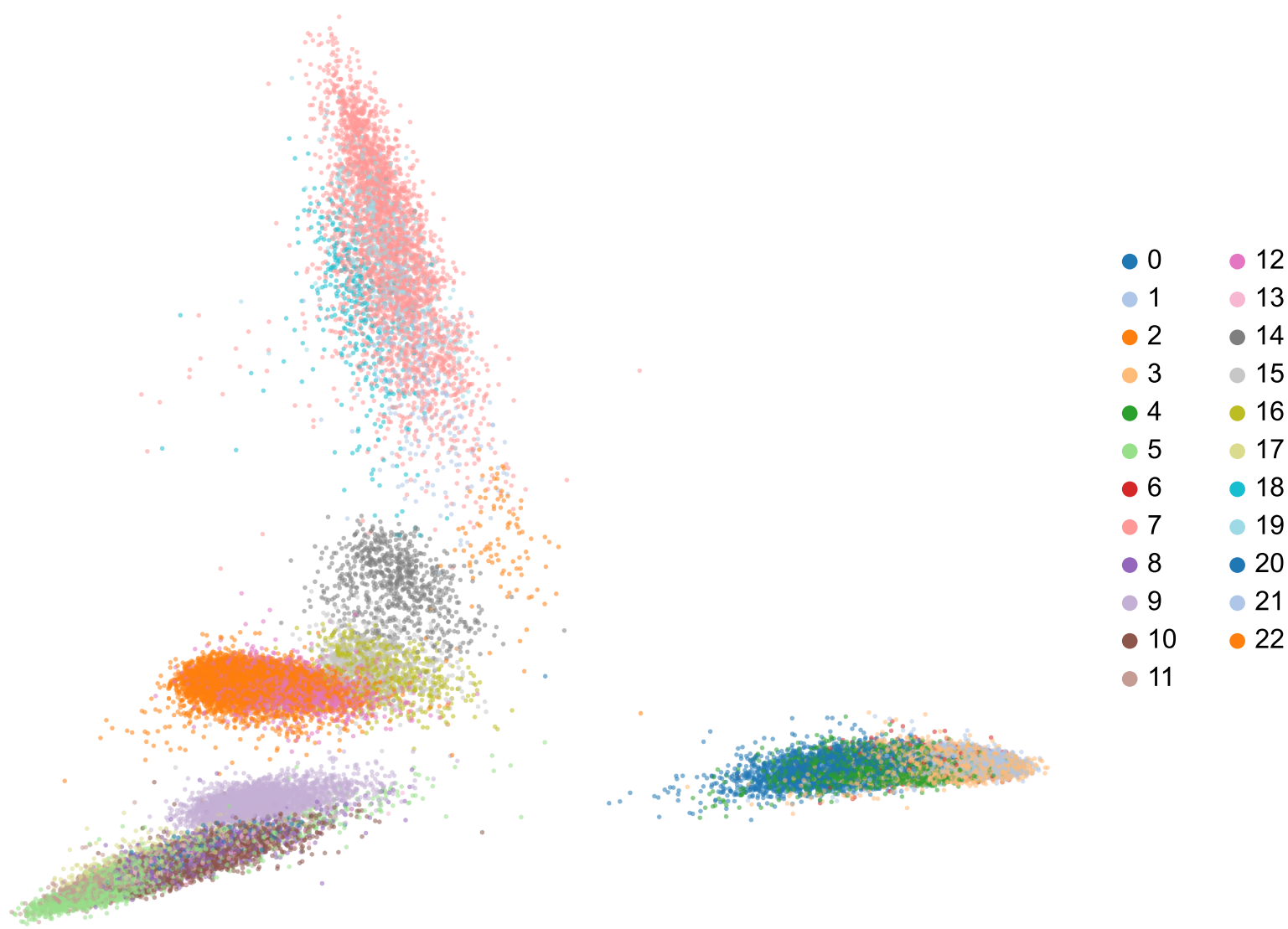
PCA colored by Leiden clusters
