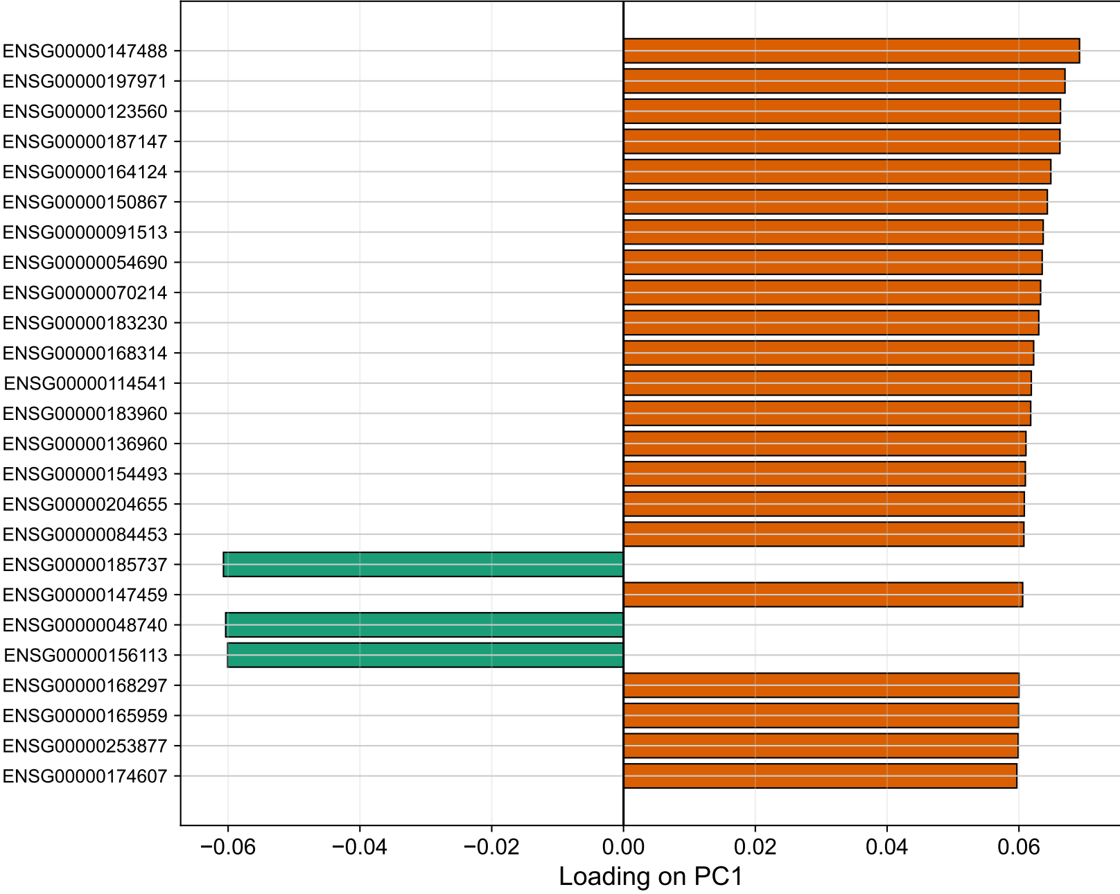
Top 25 Gene Loadings (PC1)
