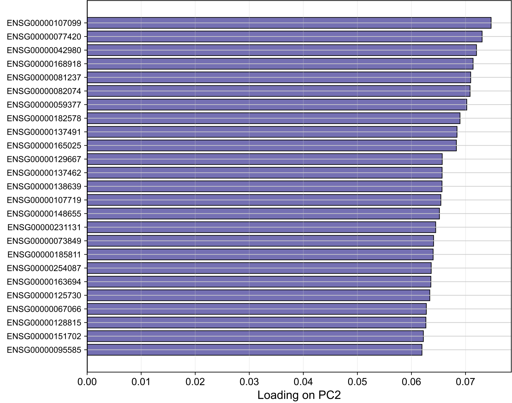
Top 25 Gene Loadings (PC2)
