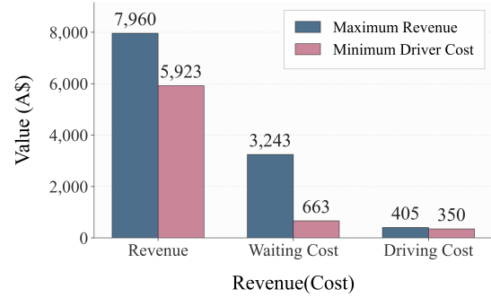
Fig. A.2. Comparison of provider revenue and driver costs under the provider-oriented and driver-oriented objectives with 50% of the baseline EV demand.
