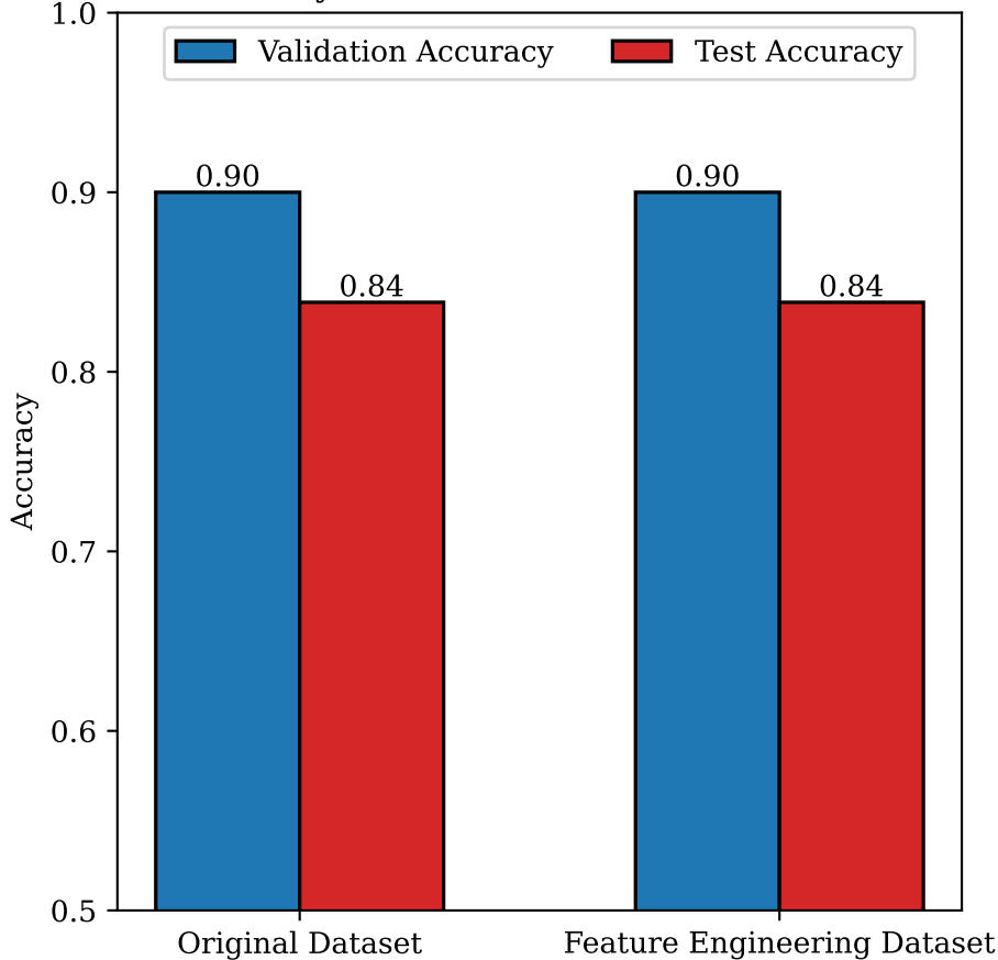
Accuracy on Validation and Test Datasets
