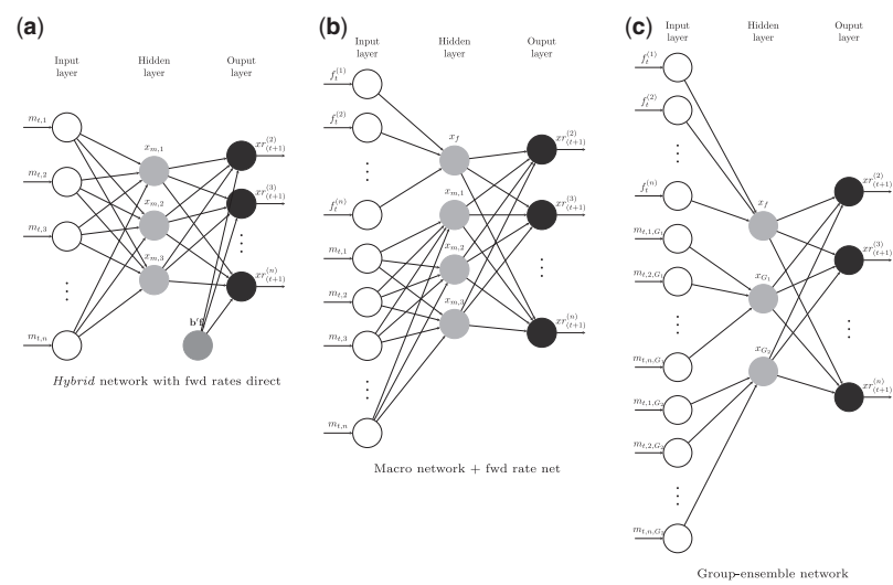
Figure 3 Examples of neural networks with forward rates and macro variables
