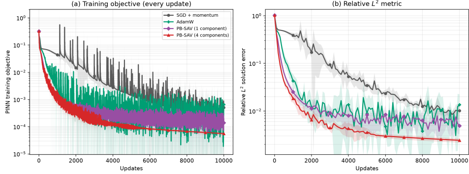
Figure 6: Five-seed comparison for the forward Burgers PINN. (a) Mean common task objective, recorded at every update, and (b) mean relative L^2 solution error. Shaded regions show one sample standard deviation.
