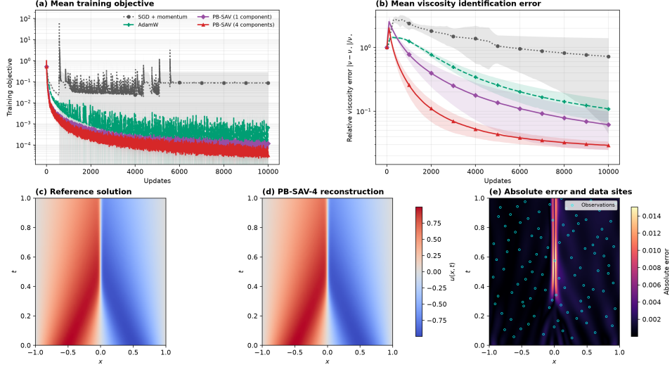
Figure 7: Five-seed comparison for inverse Burgers identification. (a) Mean common task objective and (b) mean relative viscosity error; shaded regions show one sample standard deviation. The lower row uses seed 42, the median four-component PB-SAV seed according to final viscosity error: (c) reference solution, (d) four-component PB-SAV reconstruction, and (e) absolute error with the 100 observation locations.
