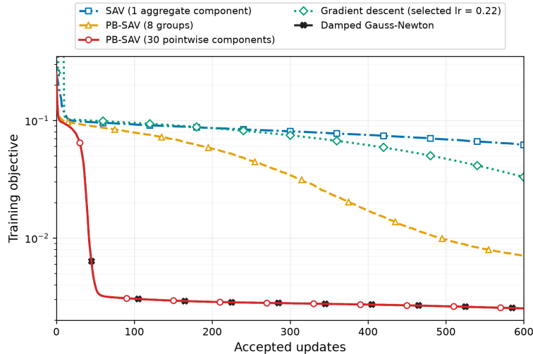
Figure 3: Training objective for one, eight, and 30 PB-SAV components, together with gradient descent and damped Gauss-Newton. The pointwise PB-SAV and Gauss-Newton trajectories are indistinguishable at plotting resolution.
