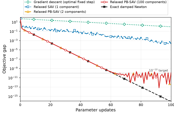
Figure 1: Convergence on the quadratic problem during the first 100 updates. All methods start from the same state.
