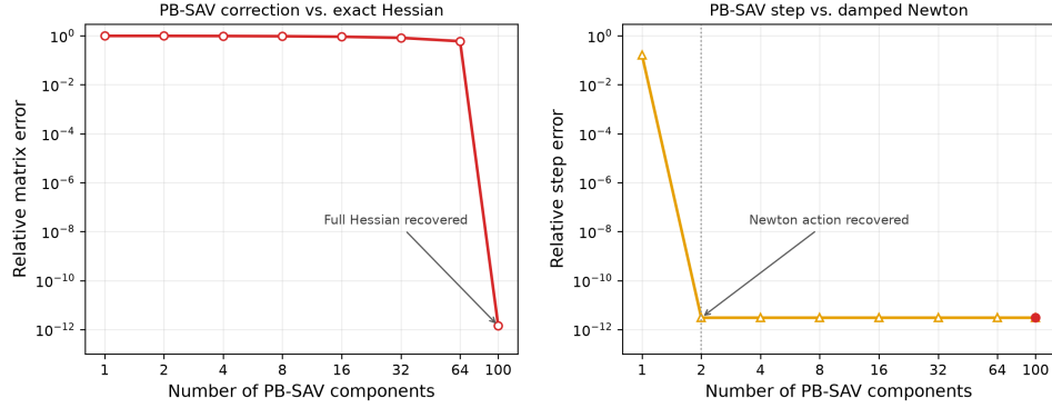
Figure 2: Fixed-state geometry for the quadratic problem. Left: relative error between the PB-SAV correction and the exact Hessian. Right: relative error between the PB-SAV increment and the damped Newton increment.
