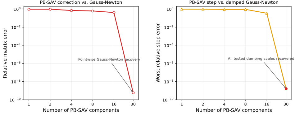
Figure 4: Fixed-state geometry for nonlinear regression. Left: relative error between the PB-SAV correction and the Gauss-Newton matrix. Right: the largest relative step error over \eta = 0.1, 1, 10, 100 . Both errors collapse when each observation is represented by a separate component.
