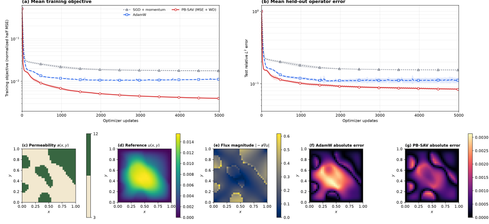
Figure 5: Five-seed Darcy DeepONet comparison. (a) Mean common training data loss and (b) mean held-out relative L^2 error; shaded regions show one sample standard deviation. The legend entry “SGD + momentum” in (a) and (b) is the full-batch heavy-ball gradient descent of Table 3. The lower row shows a fixed test sample selected by the maximum variation of the reference field: (c) permeability, (d) reference solution, (e) flux magnitude, (f) AdamW absolute error, and (g) PB-SAV absolute error.
