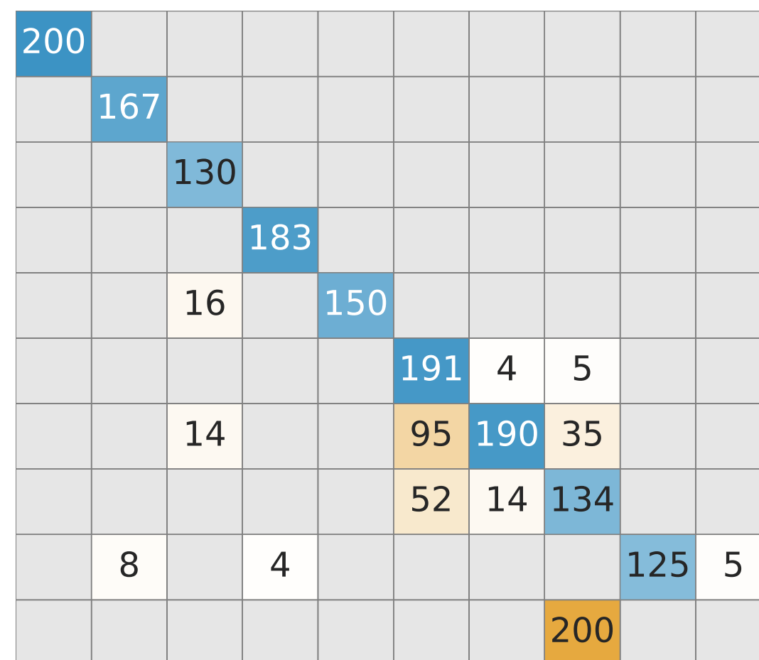
ResNet18-512-Aug870
