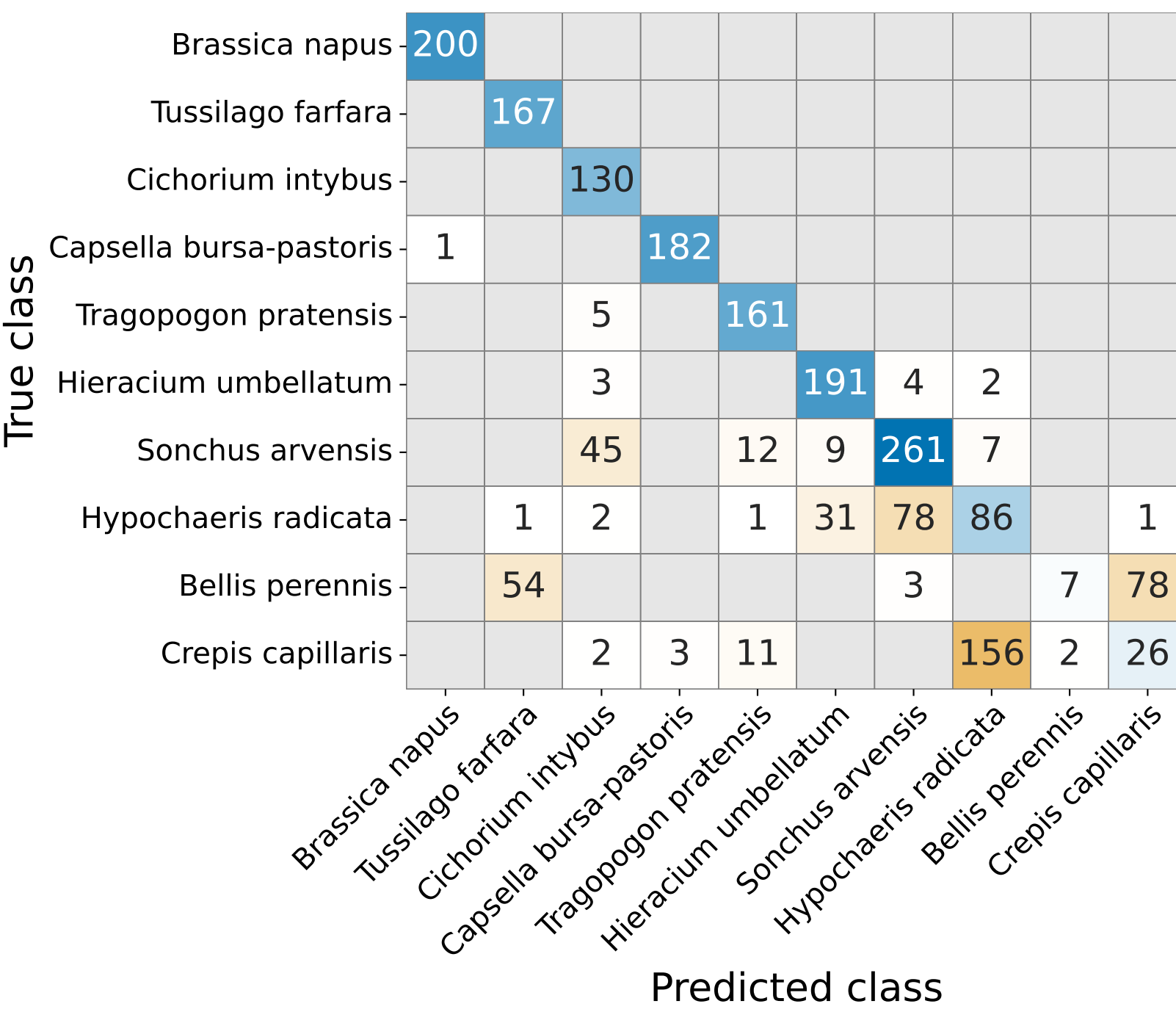
ResNet18-512-Aug1000
