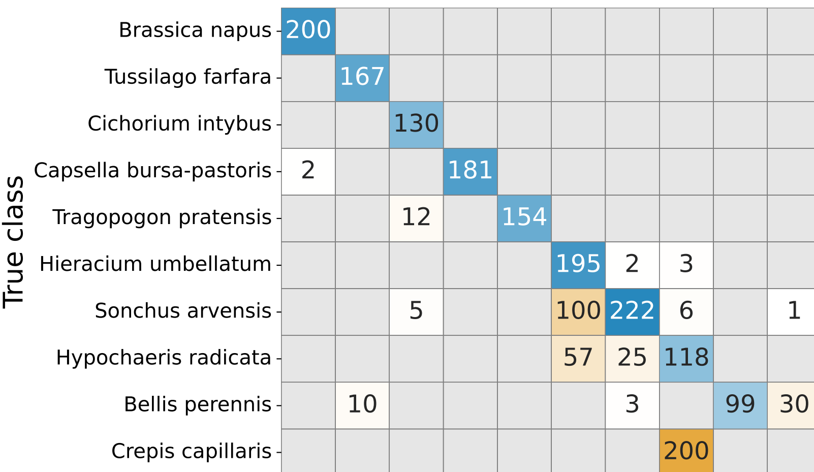
ResNet18-512-Aug1000
