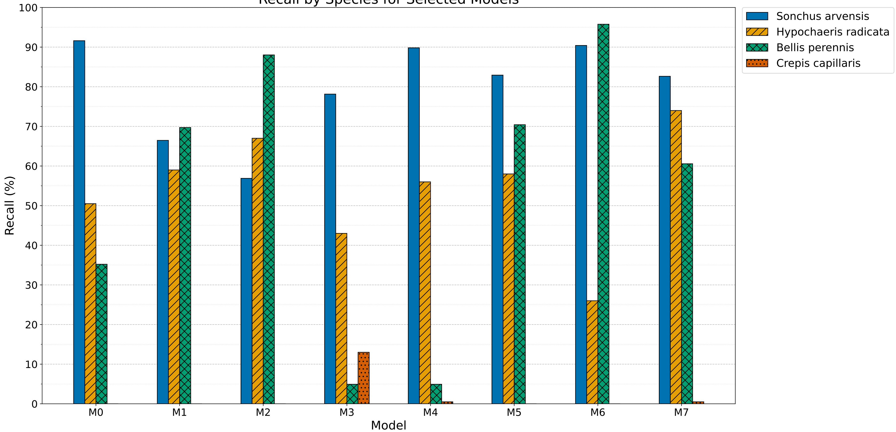
Recall by Species for Selected Models
