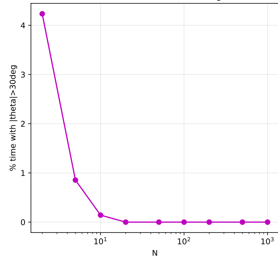
(c) Fraction in Nonlinear Range
