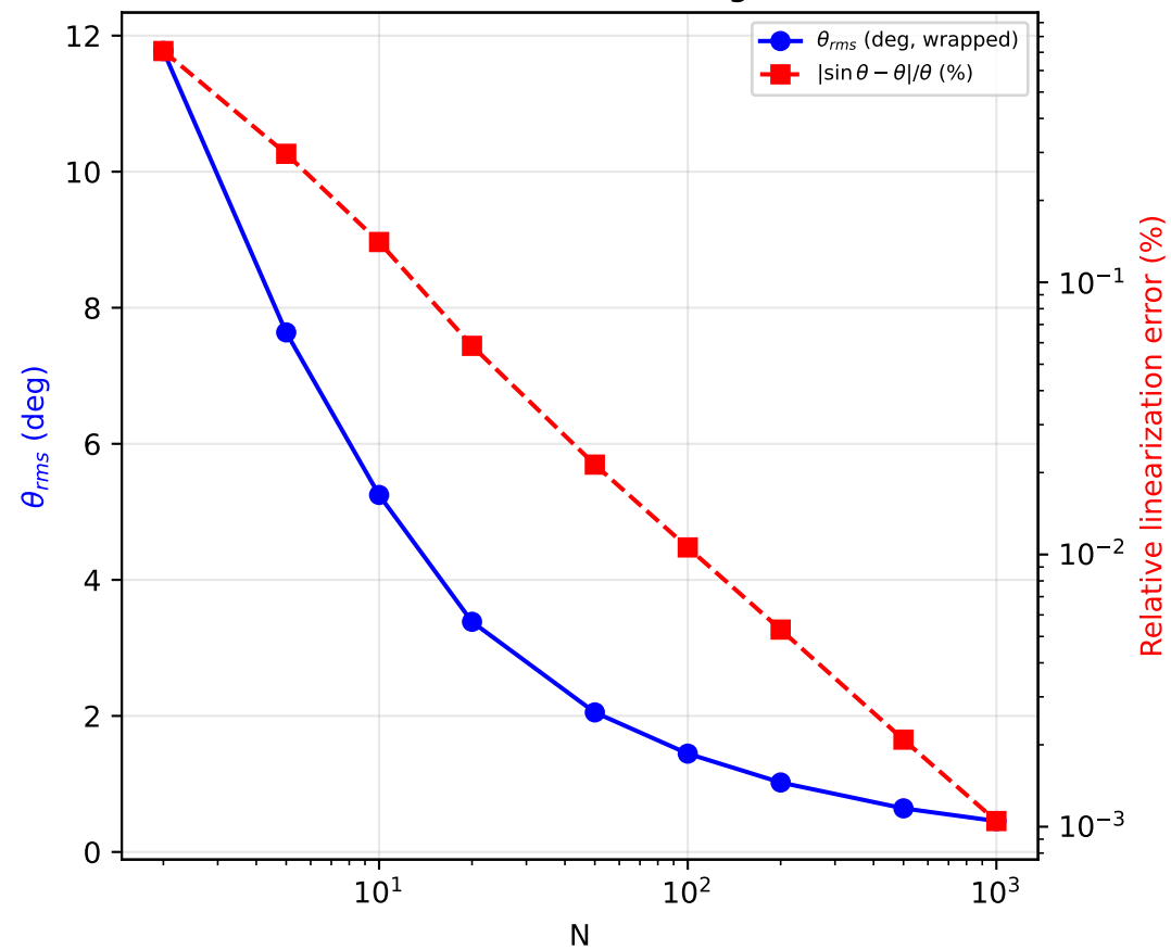
(a) Self-Linearization (bug-fixed)
