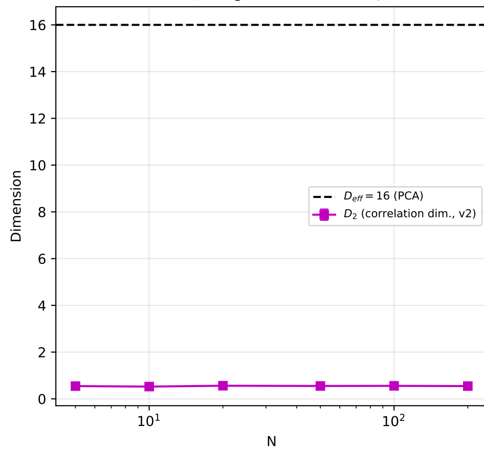
(e) D_2 (bug-fixed) vs PCA D_{eff}
