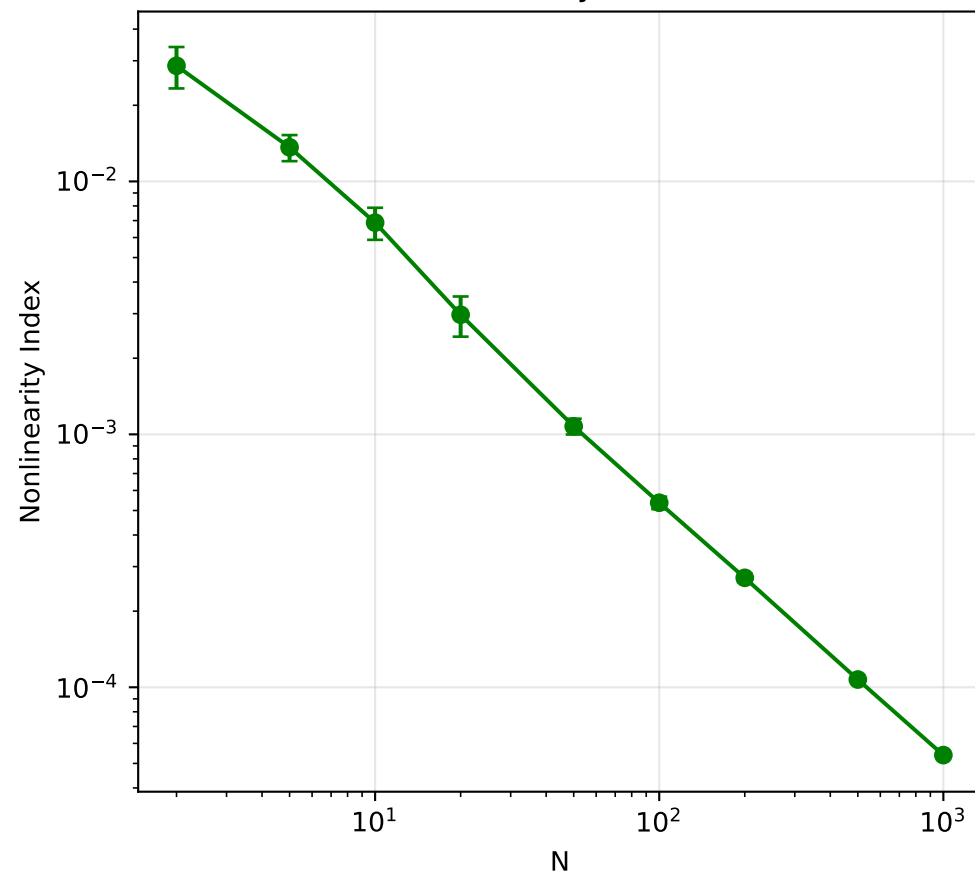
(b) Nonlinearity Index vs N
