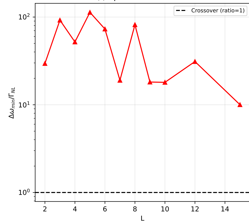
(f) Spectral Bottleneck
