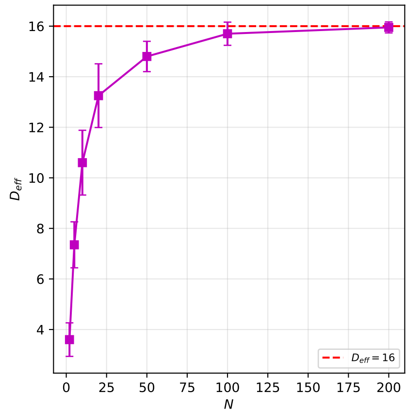
(g) D_{eff} vs N
