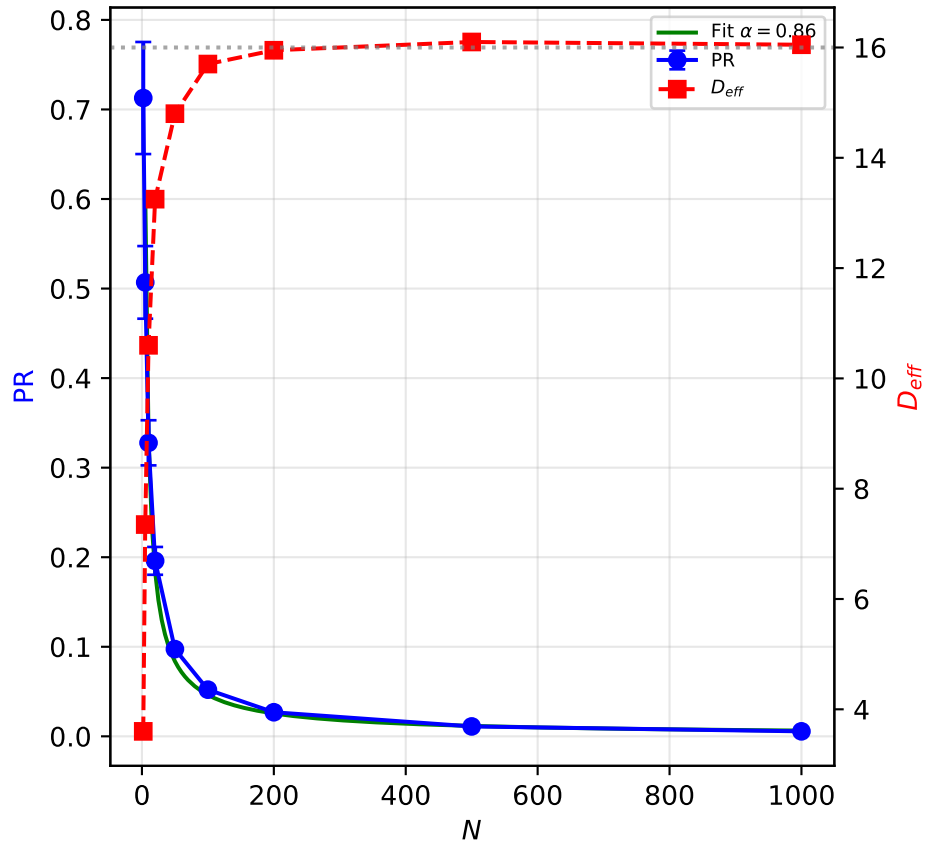
(a) 1D Scaling \alpha = 0.858
