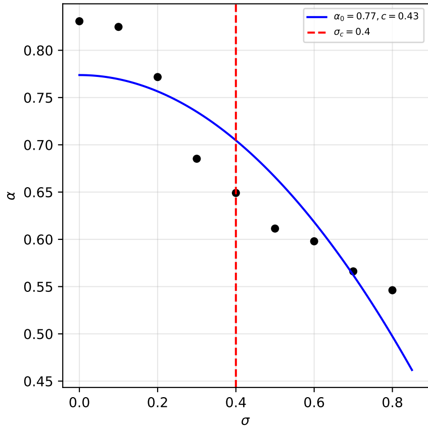
(c) Disorder Dependence
