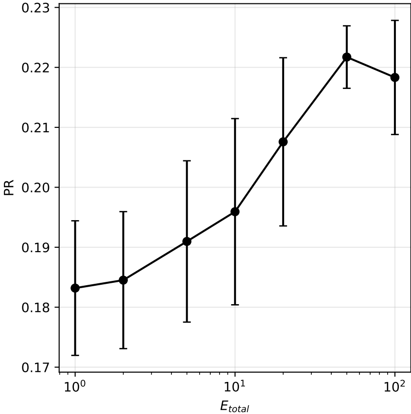
(b) Energy Sensitivity (range 19.2%, N = 20 )
