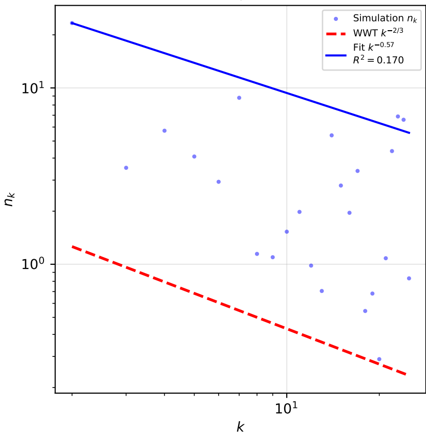
(h) KZ Spectrum
