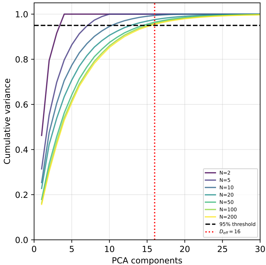
(f) D_{eff} Saturation
