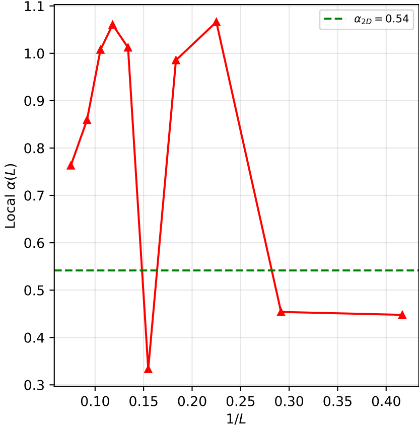
(e) 3D Finite-Size Crossover
