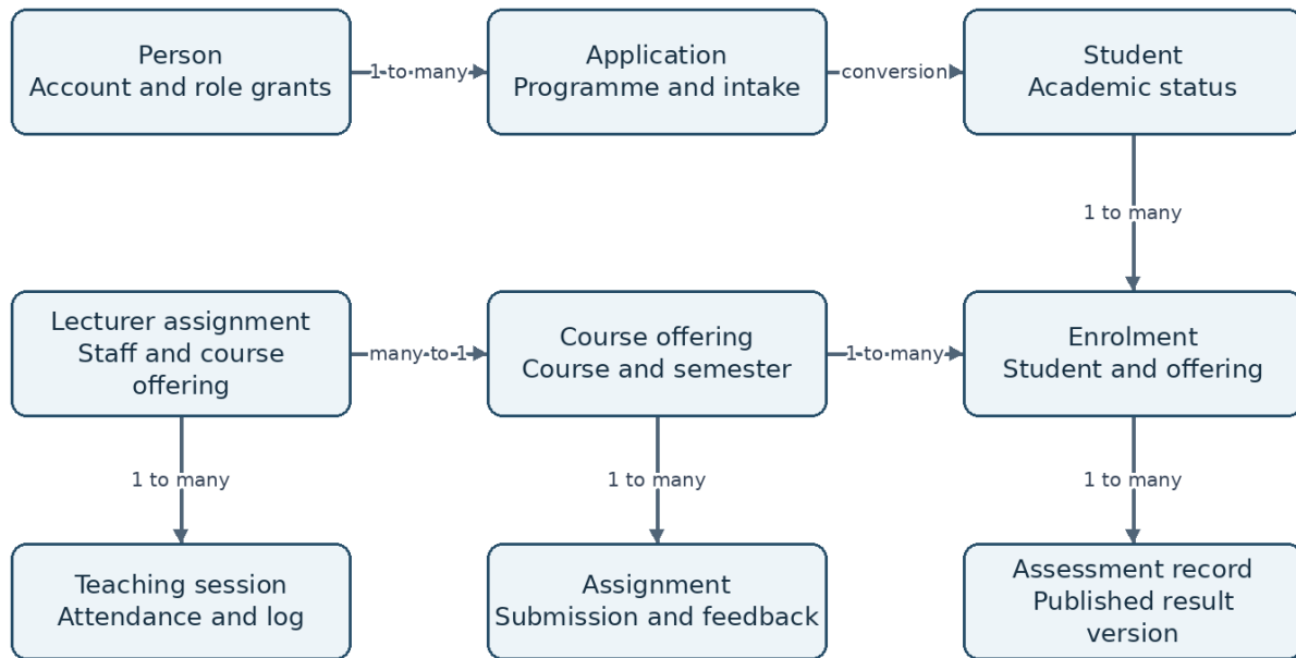
Figure 3 Principal academic entities and relationships inherited from the customer baseline.
