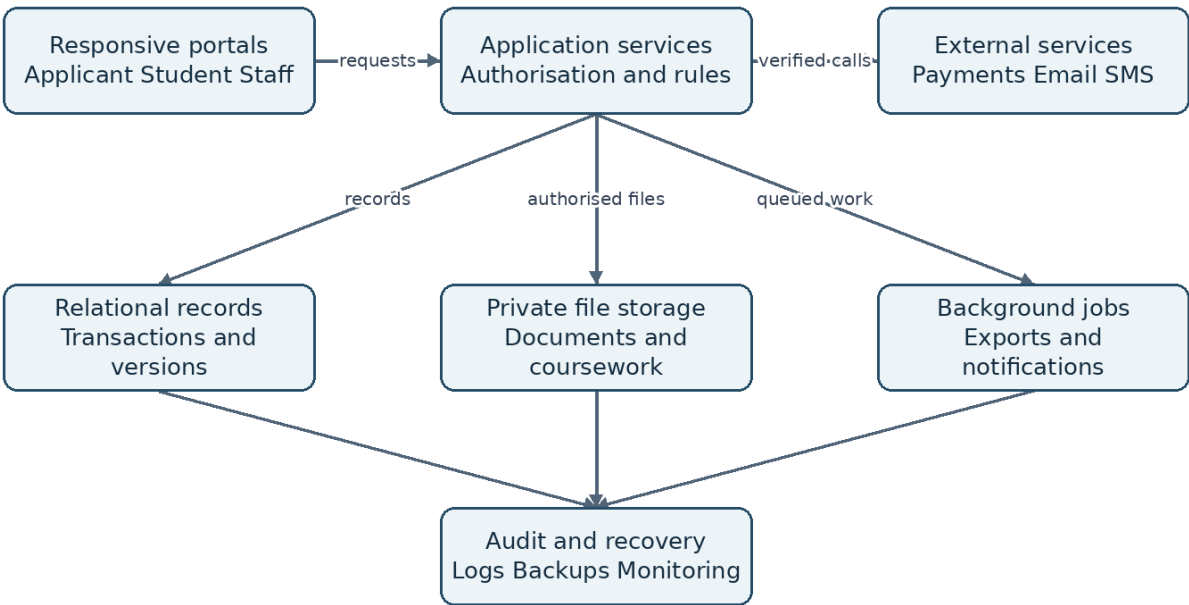
Figure 1 Logical system boundary and supporting services.
