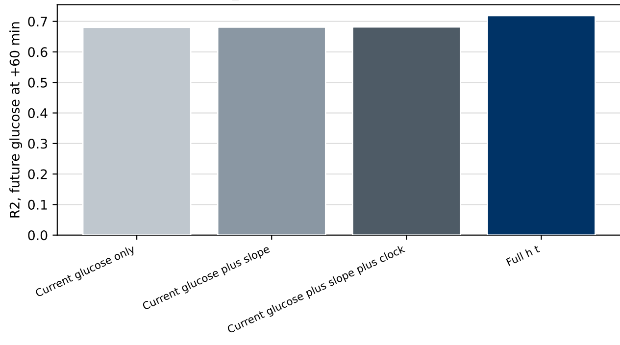
Incremental value of h_t over simple baselines
