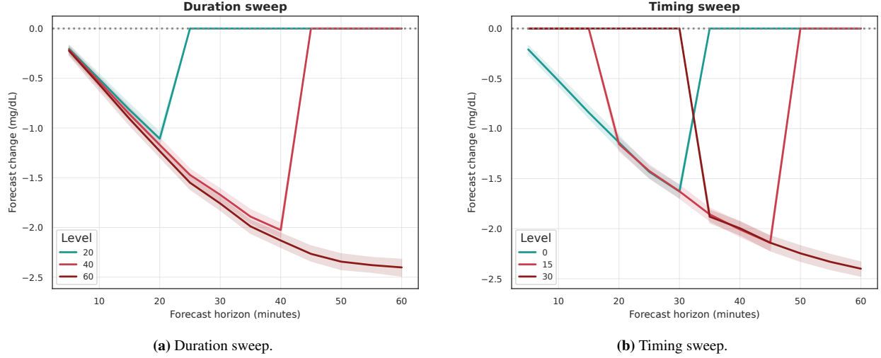
Figure 72: Temporal scenario sensitivity. Effects occur only at decoder horizons where exercise is actively supplied; no gradual post-exercise decay is propagated.
